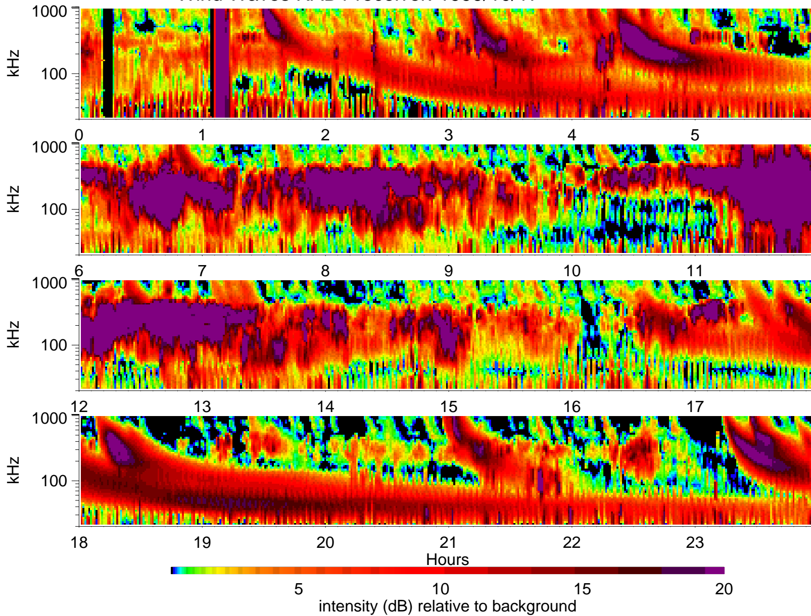
Wind Waves RAD1 receiver: 1999/10/17
