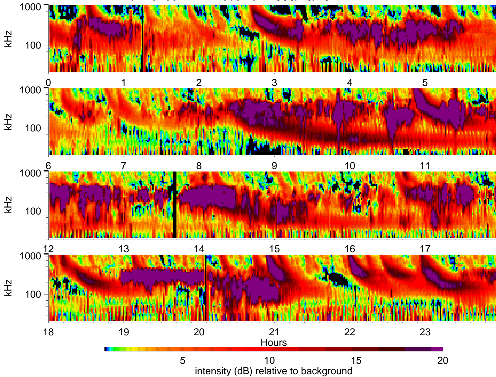
Wind Waves RAD1 receiver: 1999/10/16
