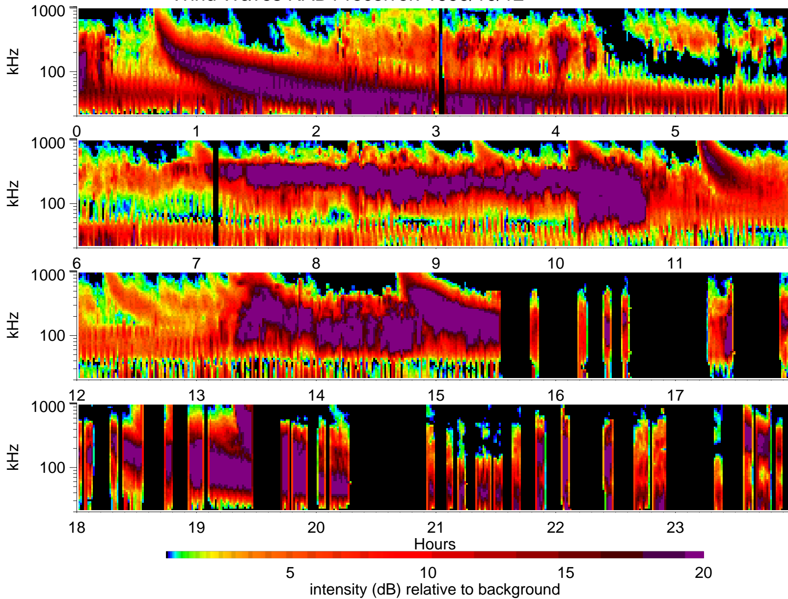
Wind Waves RAD1 receiver: 1999/10/12
