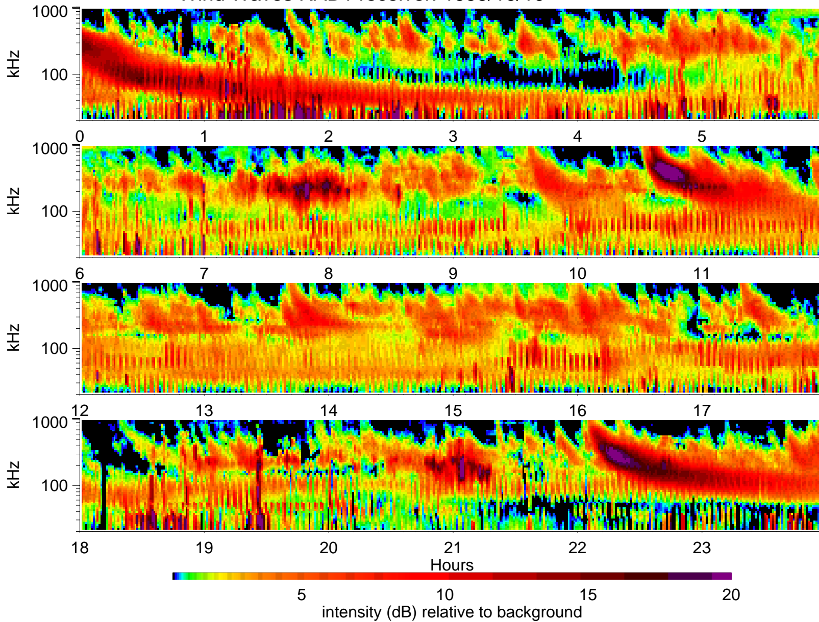
Wind Waves RAD1 receiver: 1999/10/10
