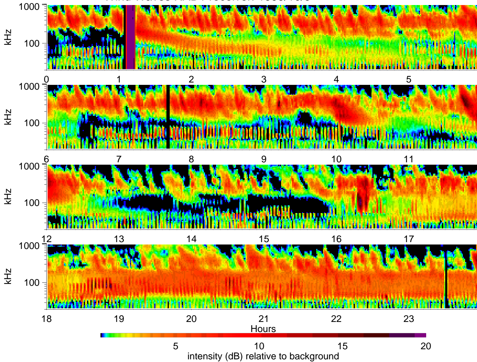
Wind Waves RAD1 receiver: 1999/10/9
