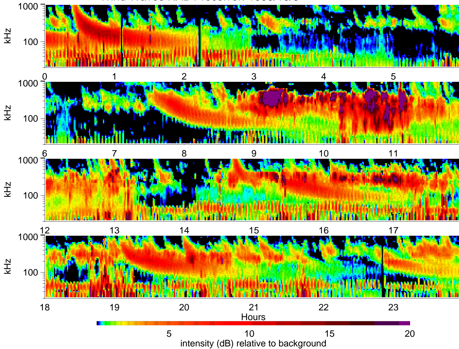
Wind Waves RAD1 receiver: 1999/10/6
