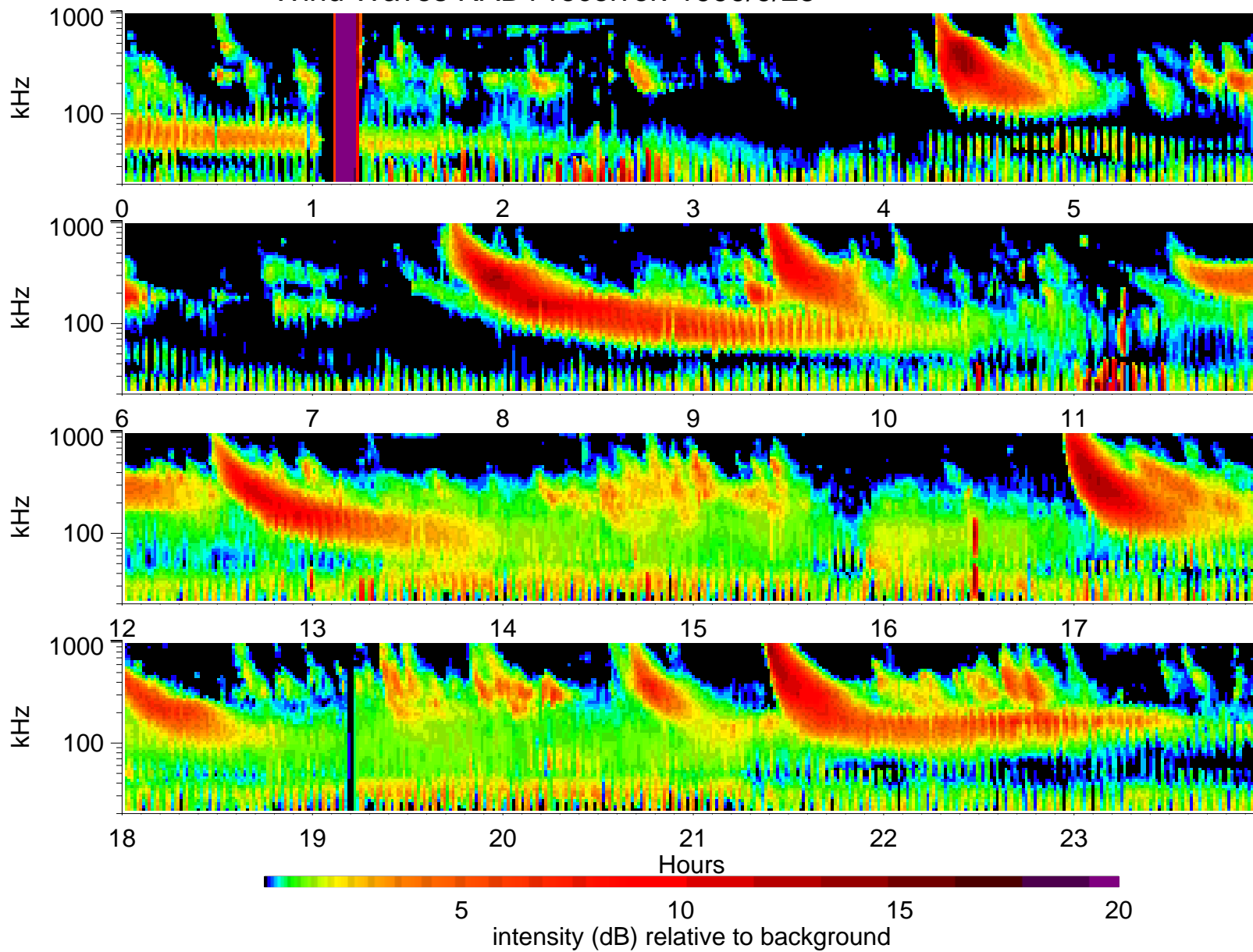
Wind Waves RAD1 receiver: 1999/9/25
