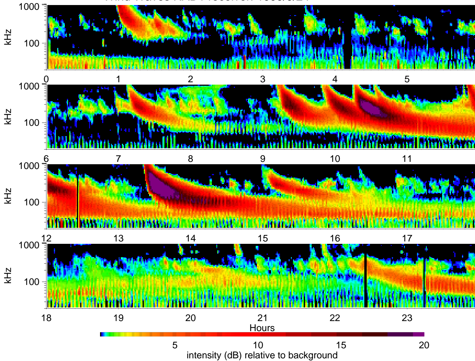
Wind Waves RAD1 receiver: 1999/9/24
