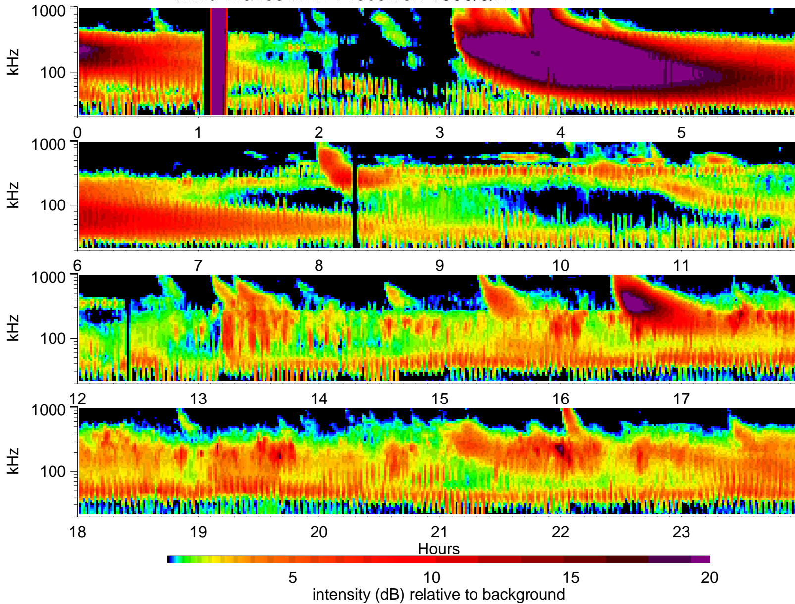
Wind Waves RAD1 receiver: 1999/9/21
