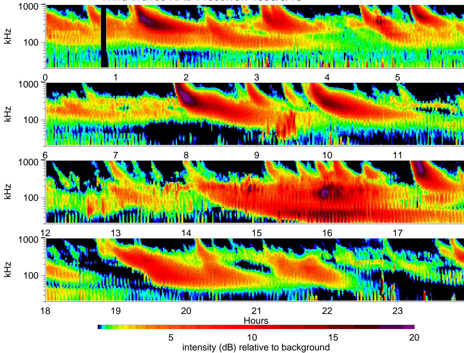
Wind Waves RAD1 receiver: 1999/9/18
