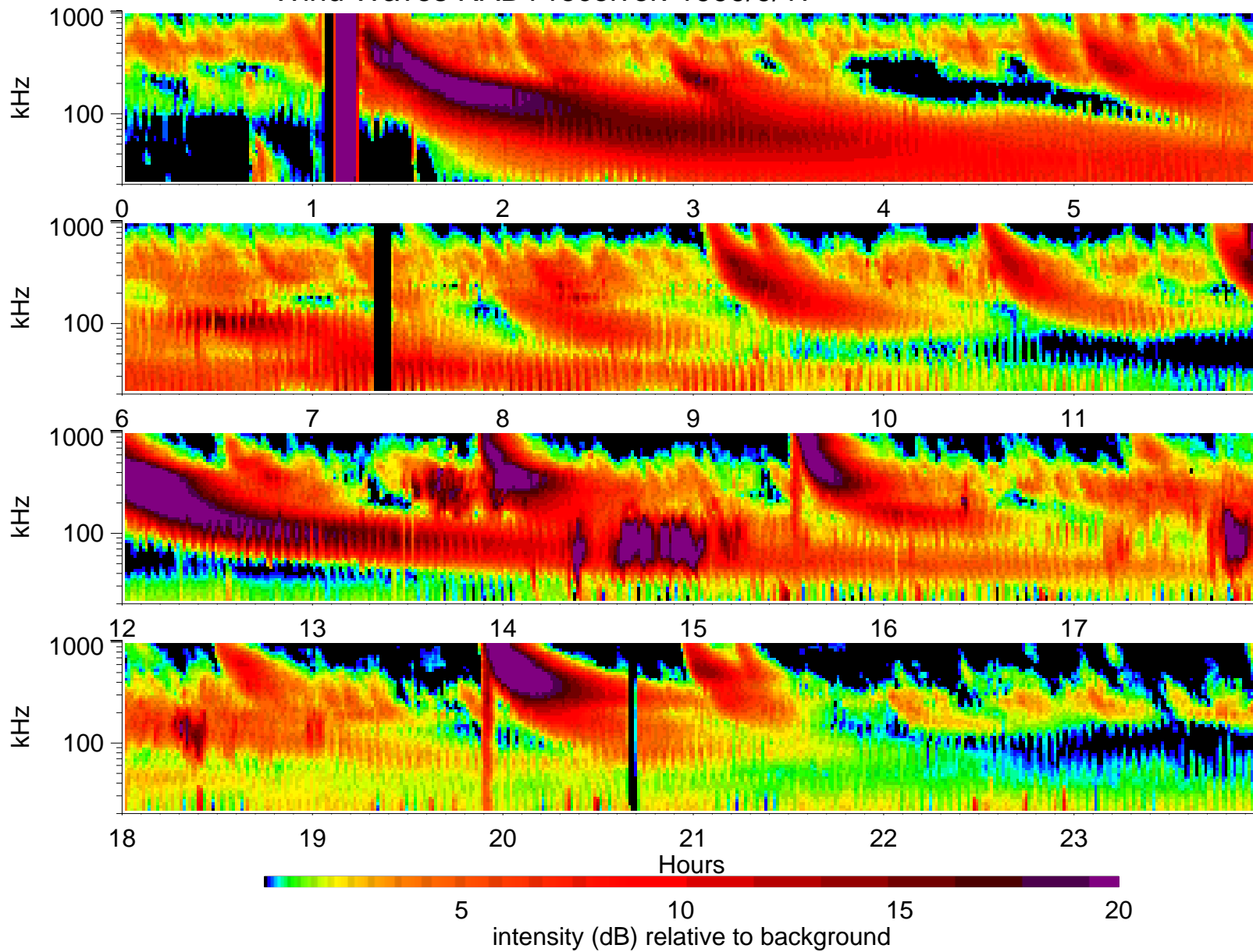
Wind Waves RAD1 receiver: 1999/9/17
