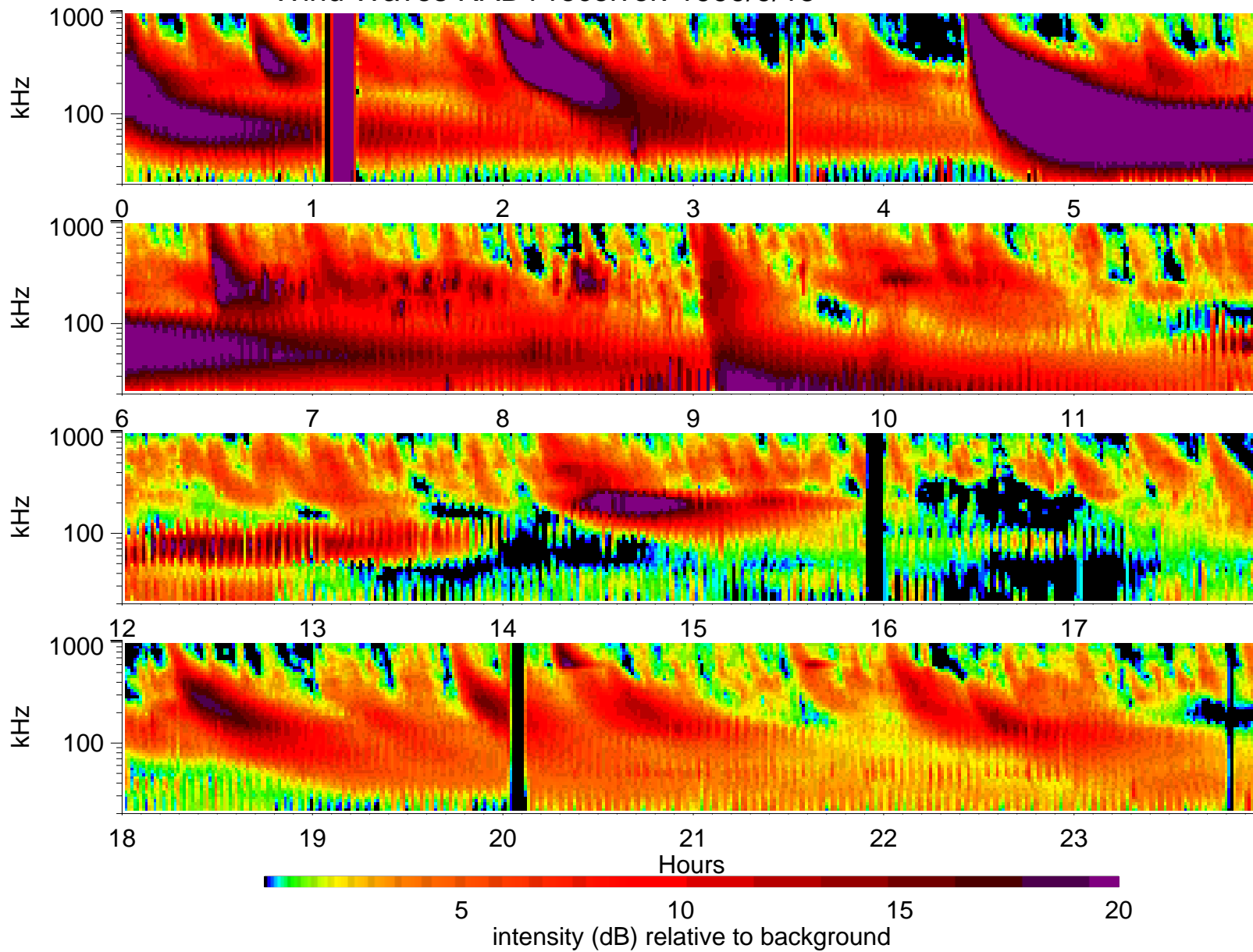
Wind Waves RAD1 receiver: 1999/9/15
