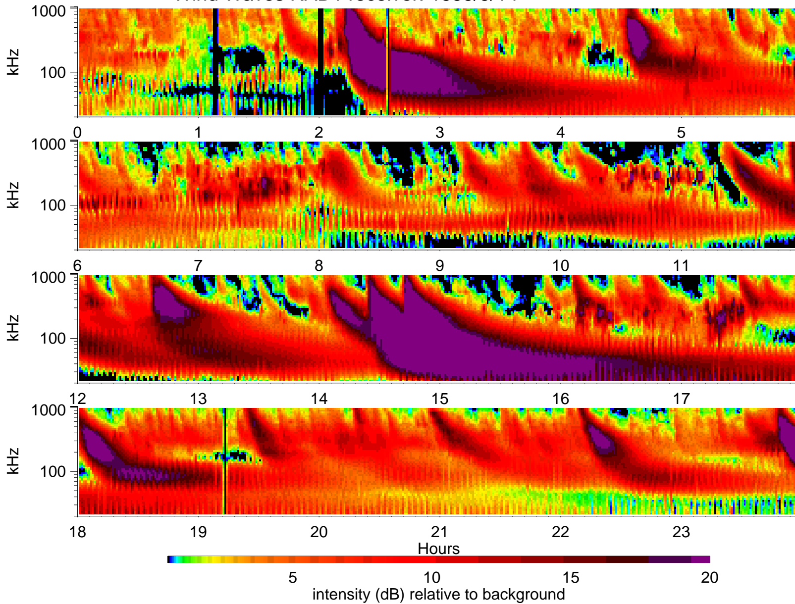
Wind Waves RAD1 receiver: 1999/9/14
