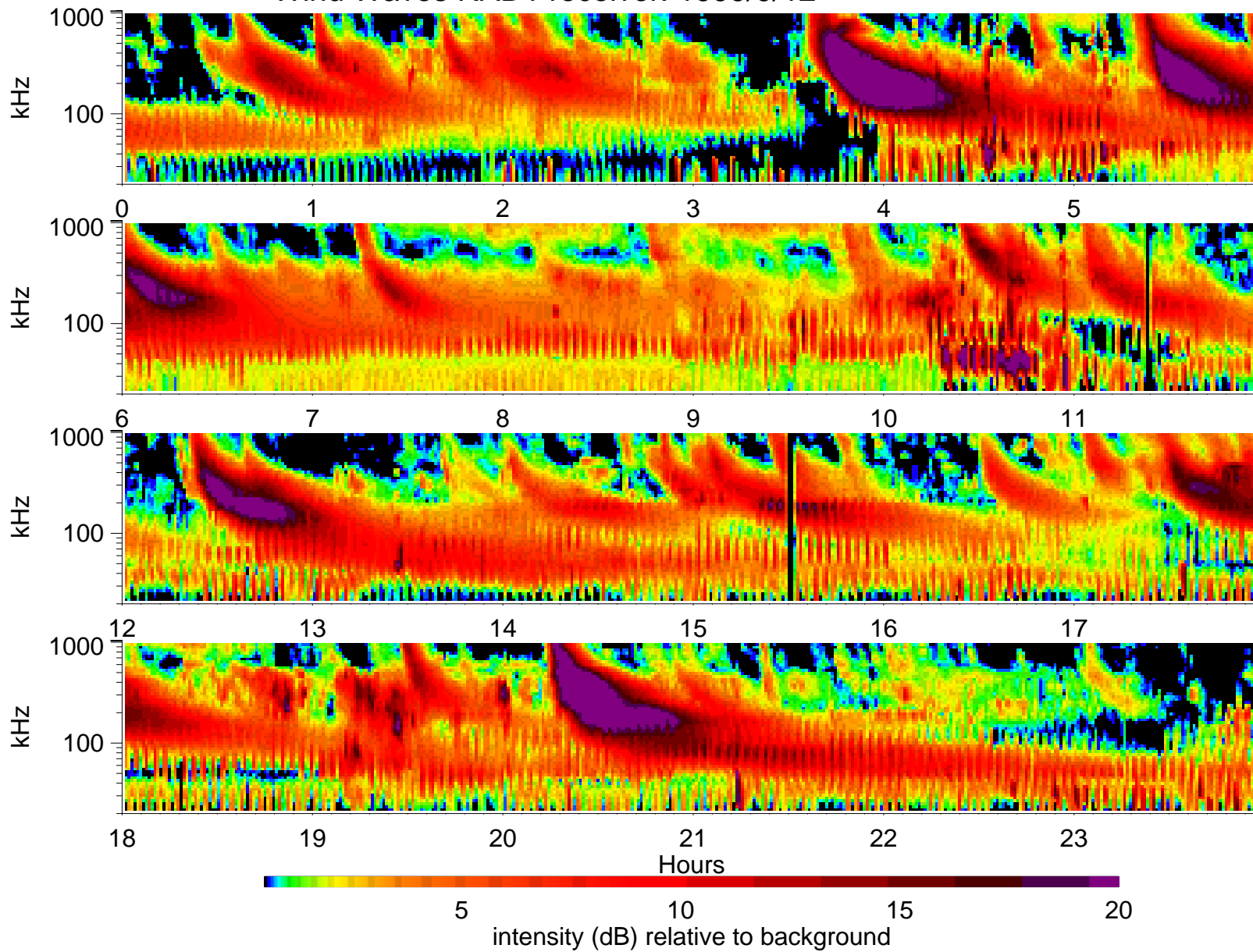
Wind Waves RAD1 receiver: 1999/9/12
