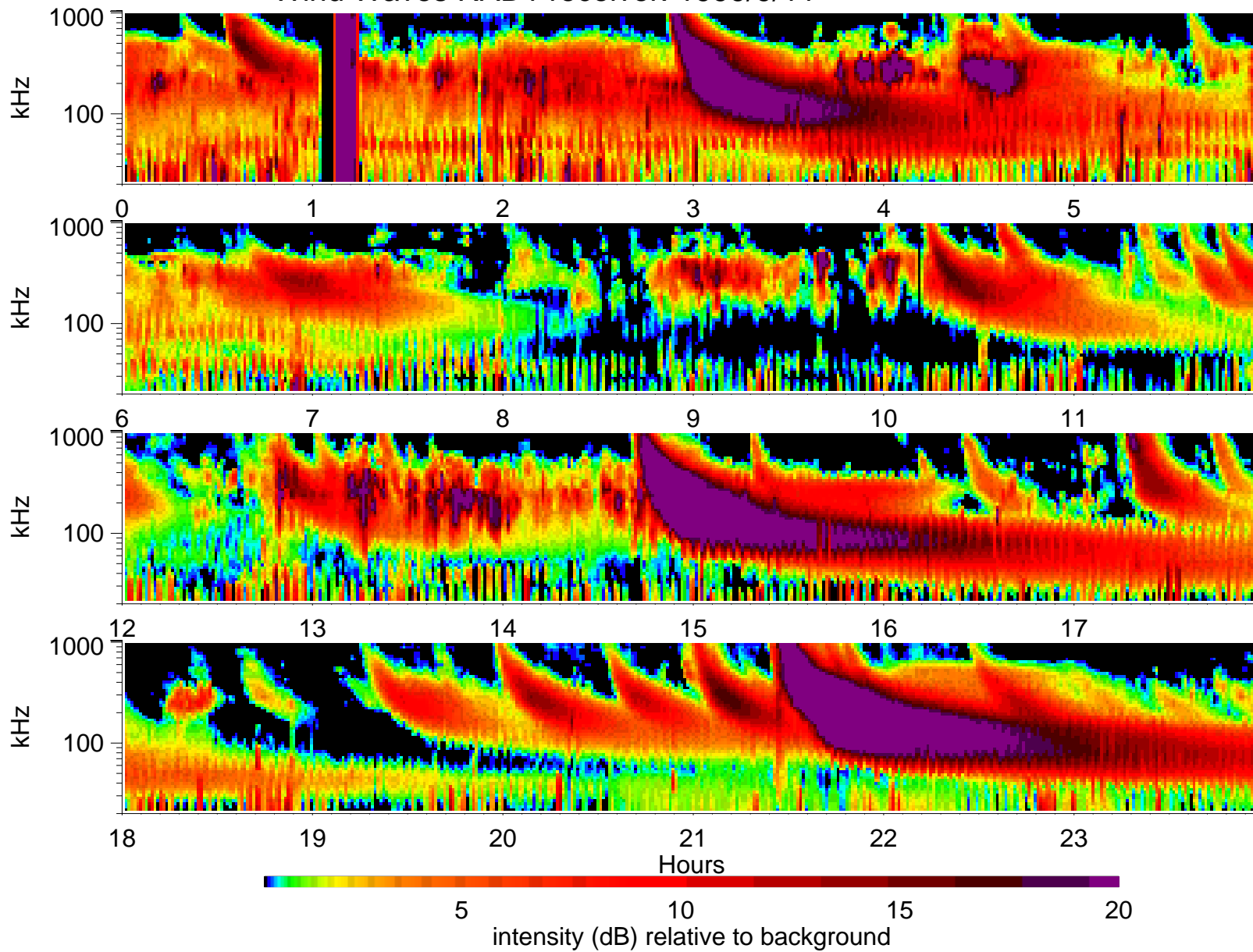
Wind Waves RAD1 receiver: 1999/9/11
