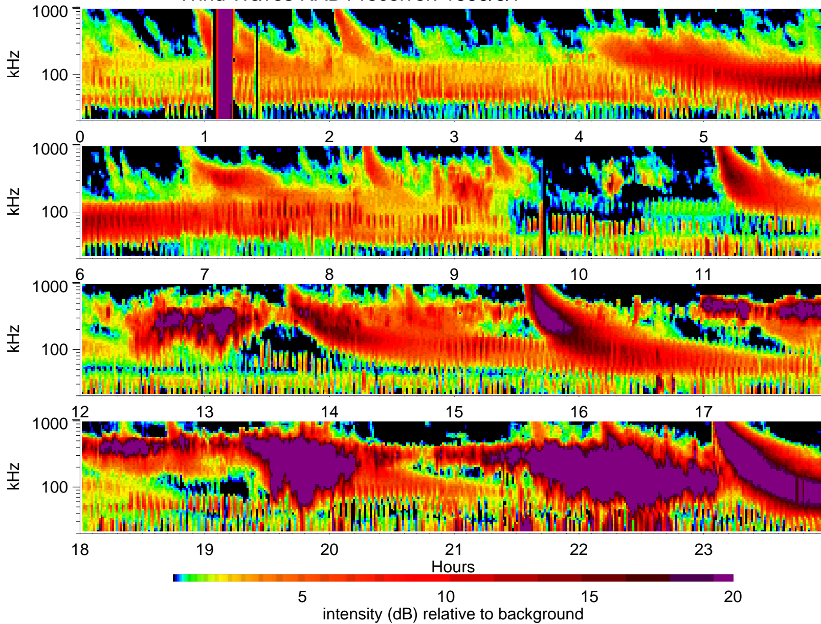
Wind Waves RAD1 receiver: 1999/9/7
