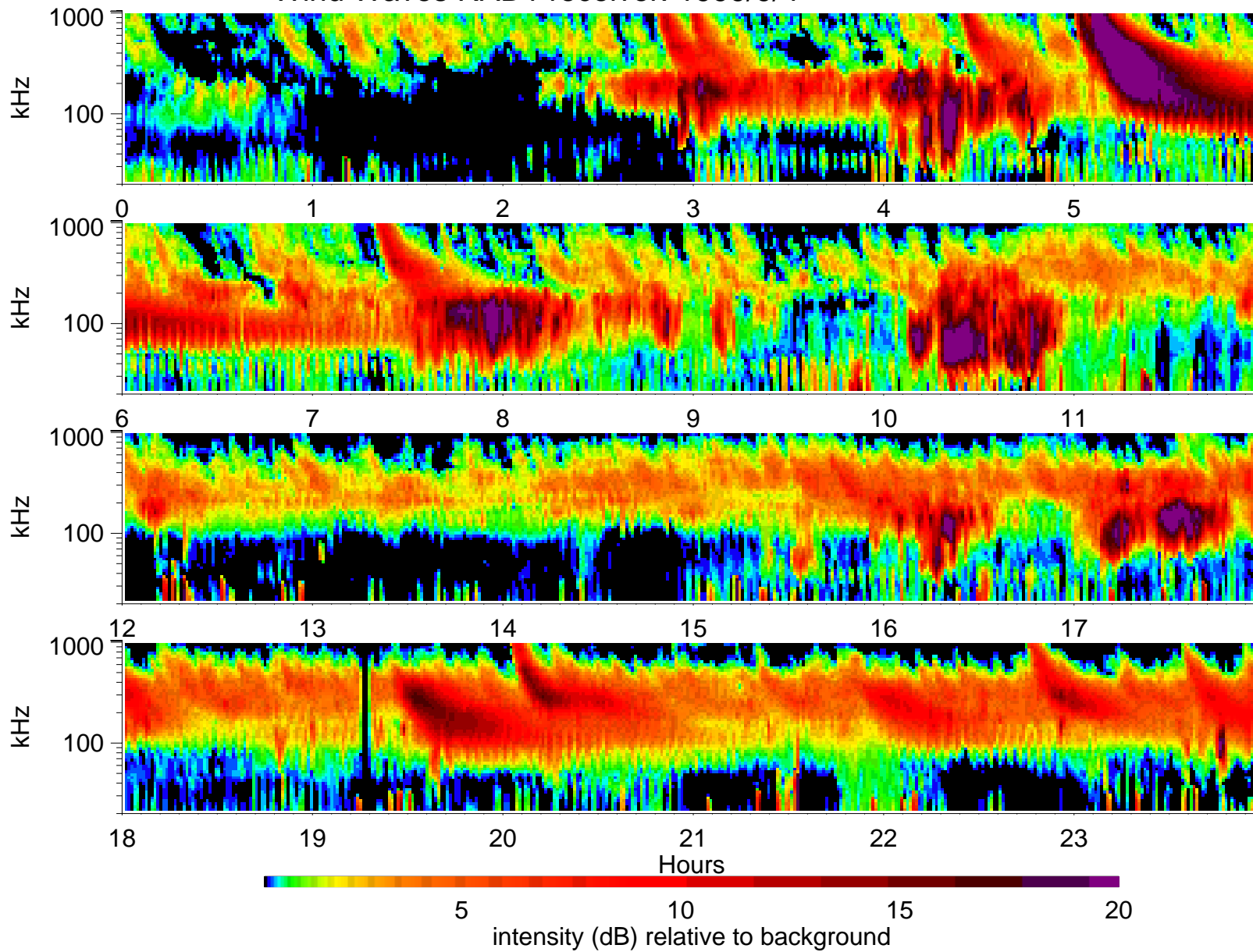
Wind Waves RAD1 receiver: 1999/9/4
