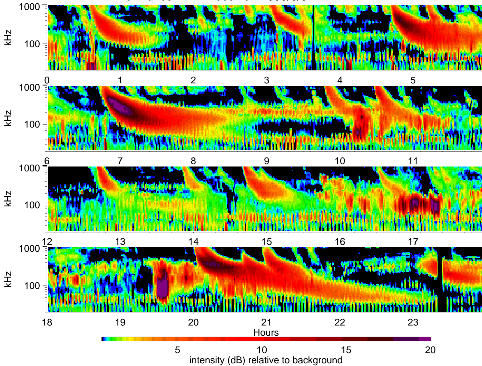
Wind Waves RAD1 receiver: 1999/8/31
