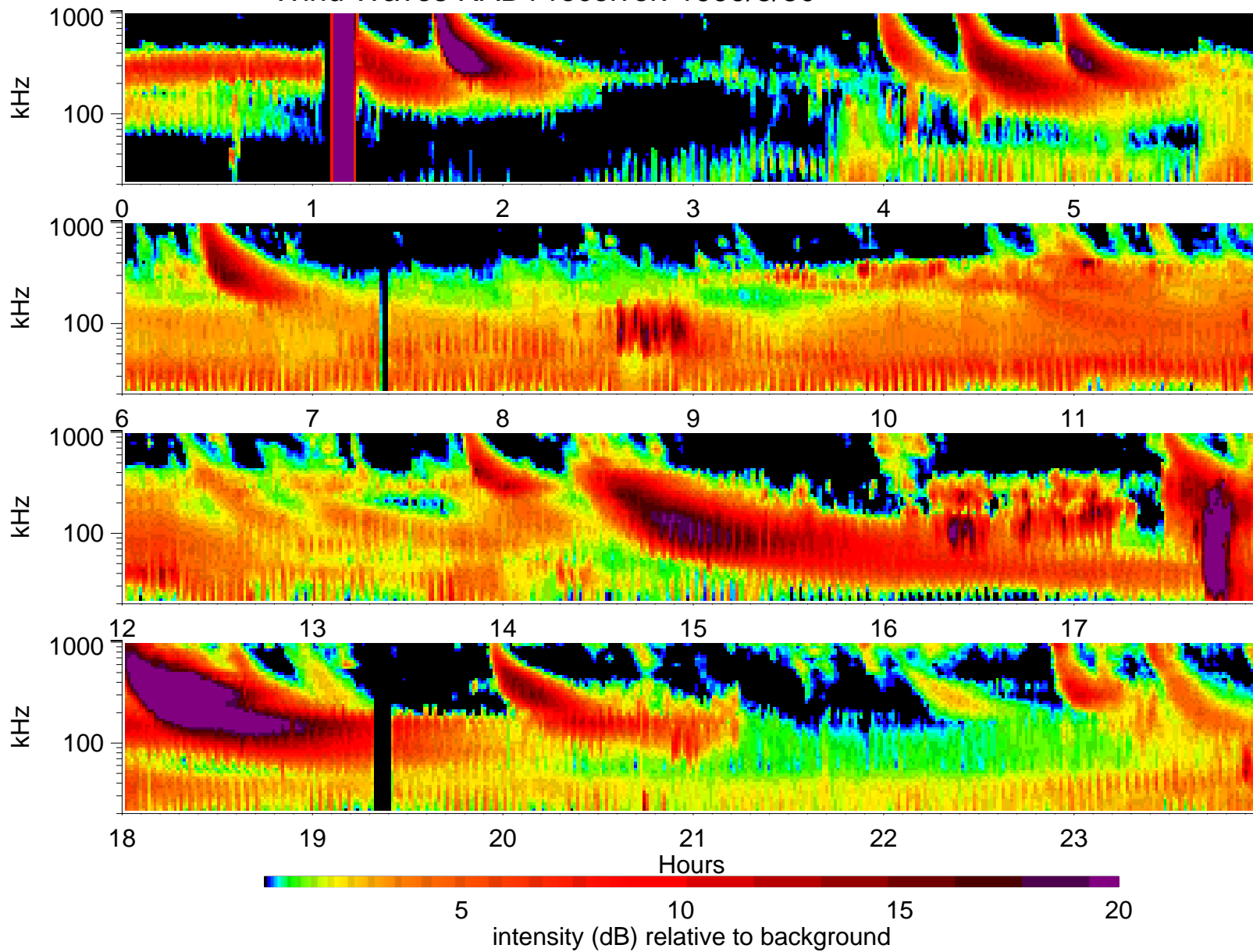
Wind Waves RAD1 receiver: 1999/8/30
