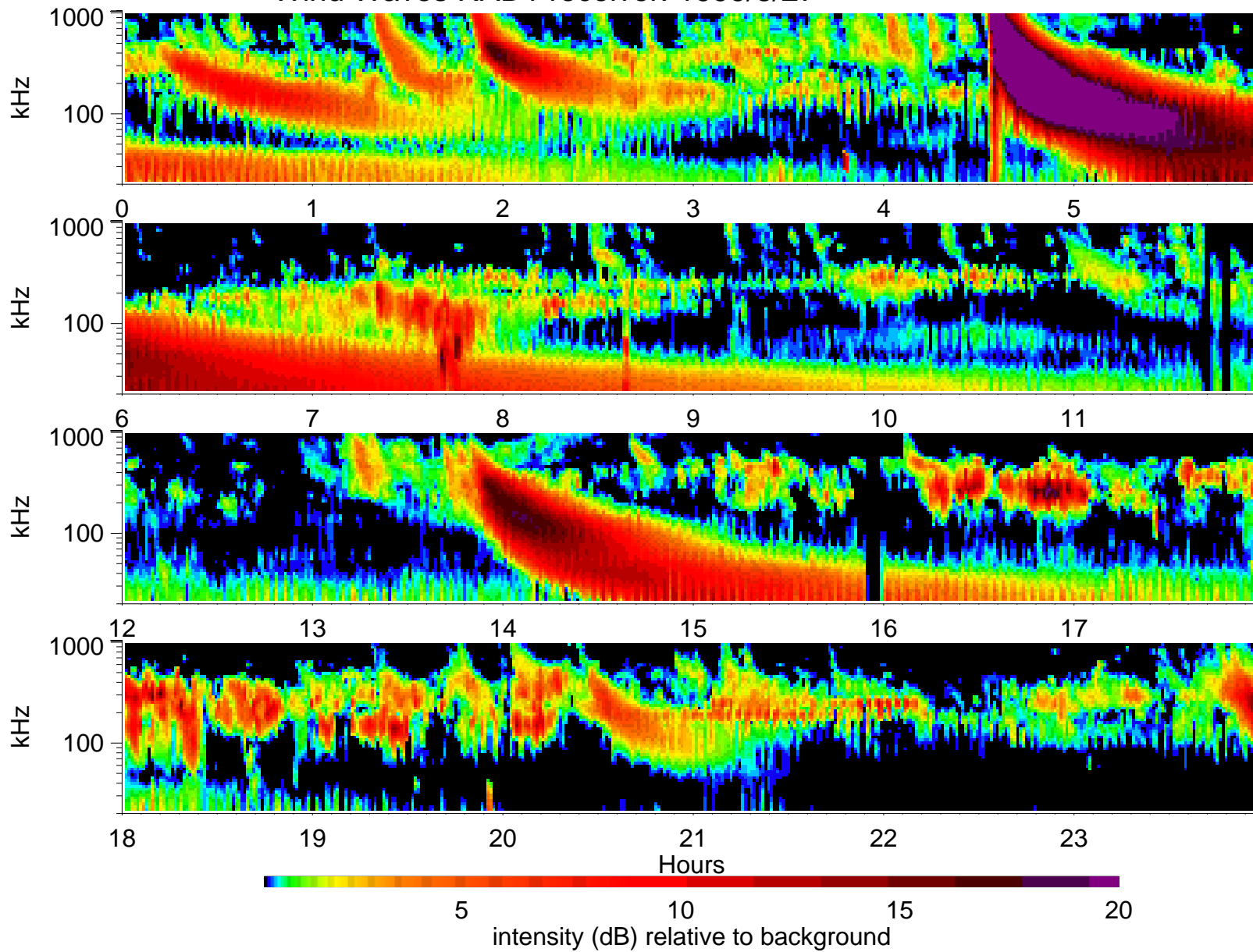
Wind Waves RAD1 receiver: 1999/8/27
