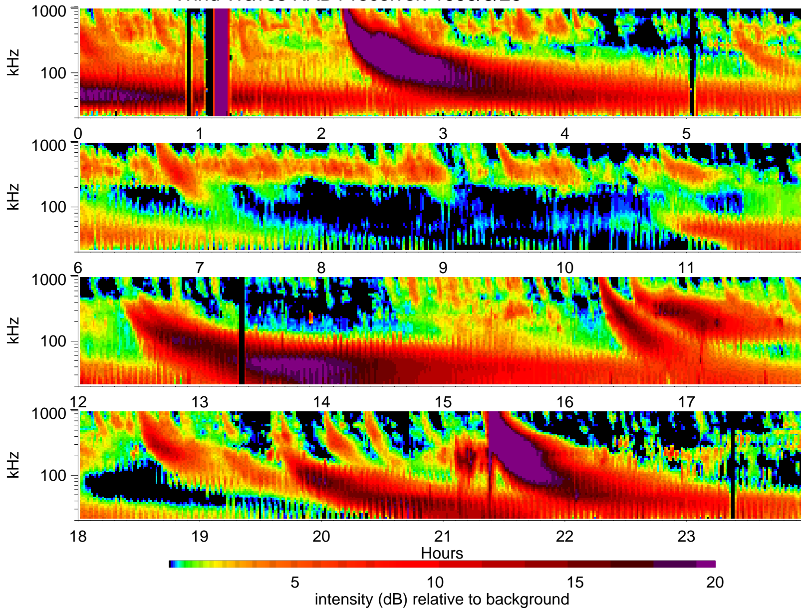
Wind Waves RAD1 receiver: 1999/8/26
