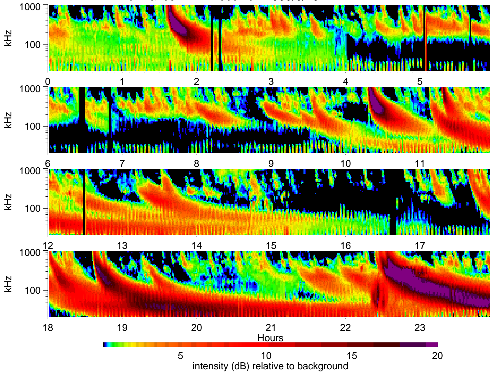
Wind Waves RAD1 receiver: 1999/8/25
