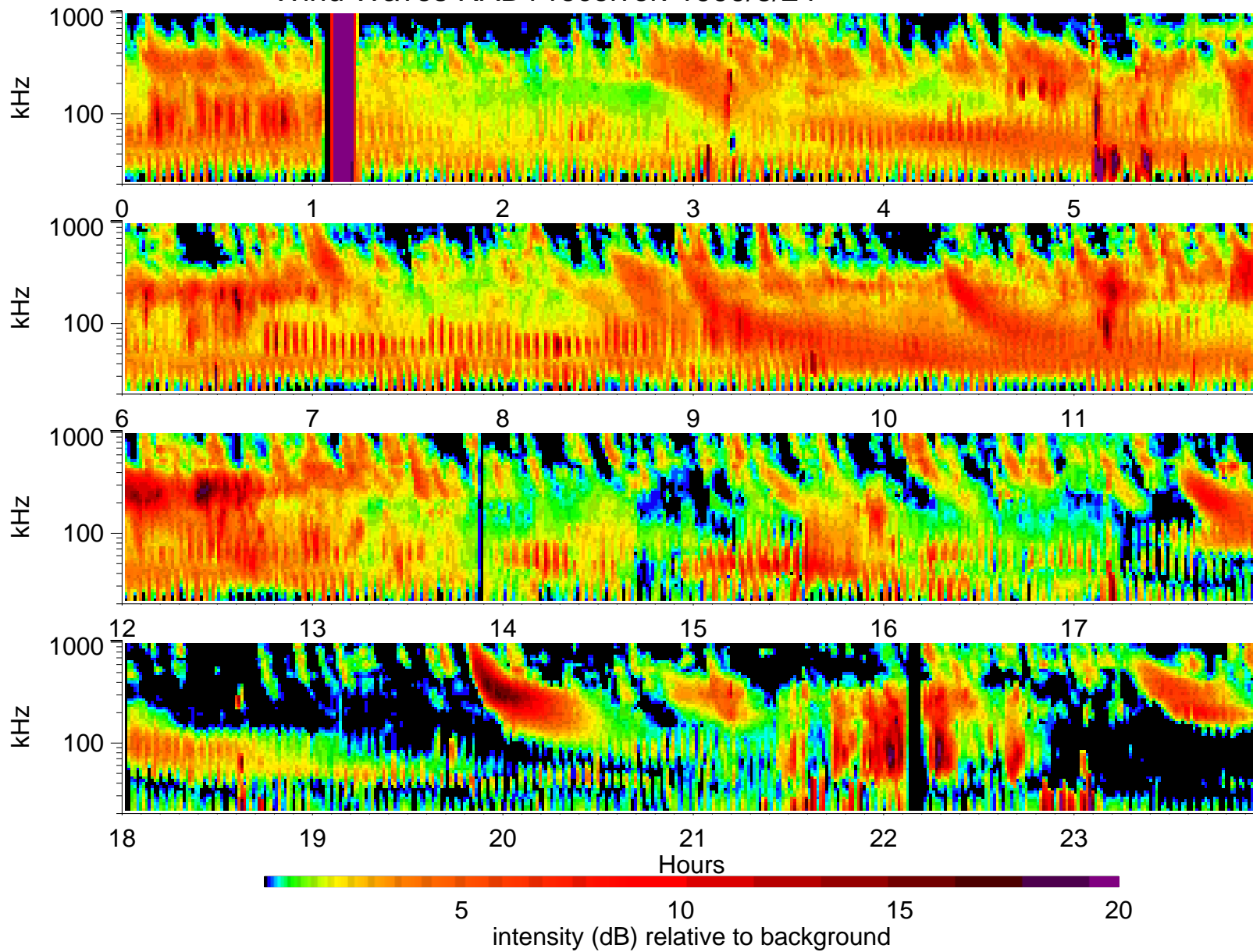
Wind Waves RAD1 receiver: 1999/8/24
