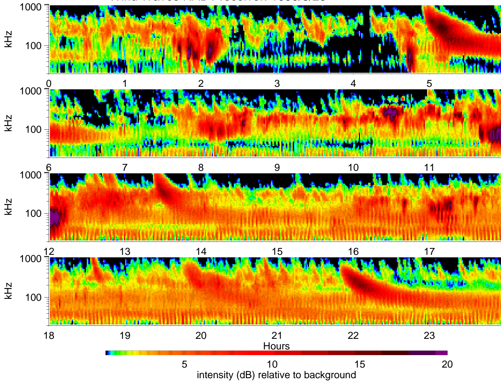
Wind Waves RAD1 receiver: 1999/8/23
