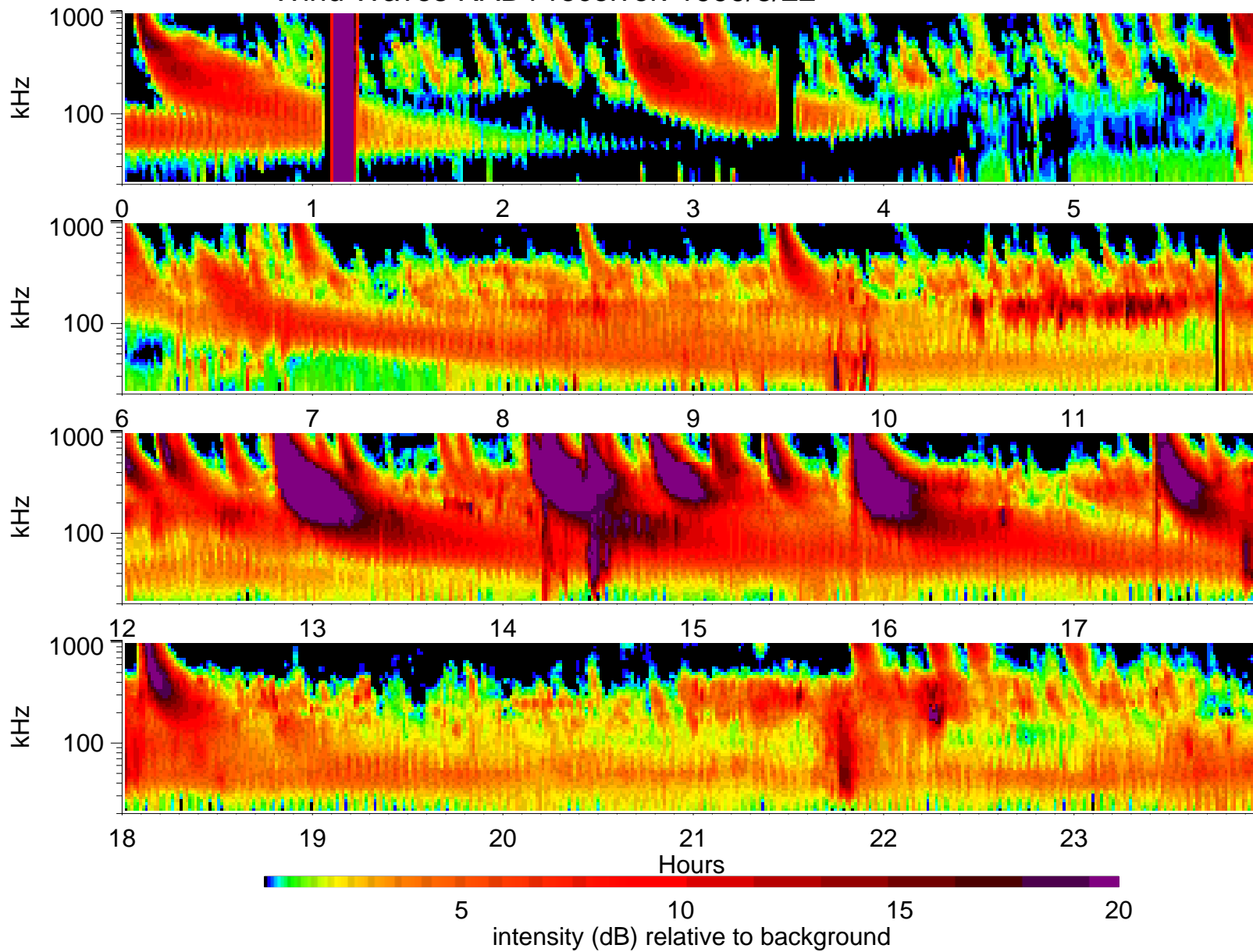
Wind Waves RAD1 receiver: 1999/8/22
