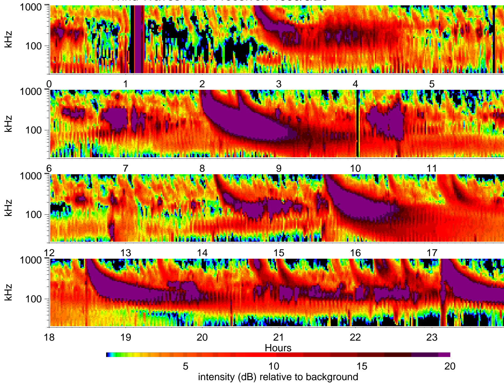
Wind Waves RAD1 receiver: 1999/8/20
