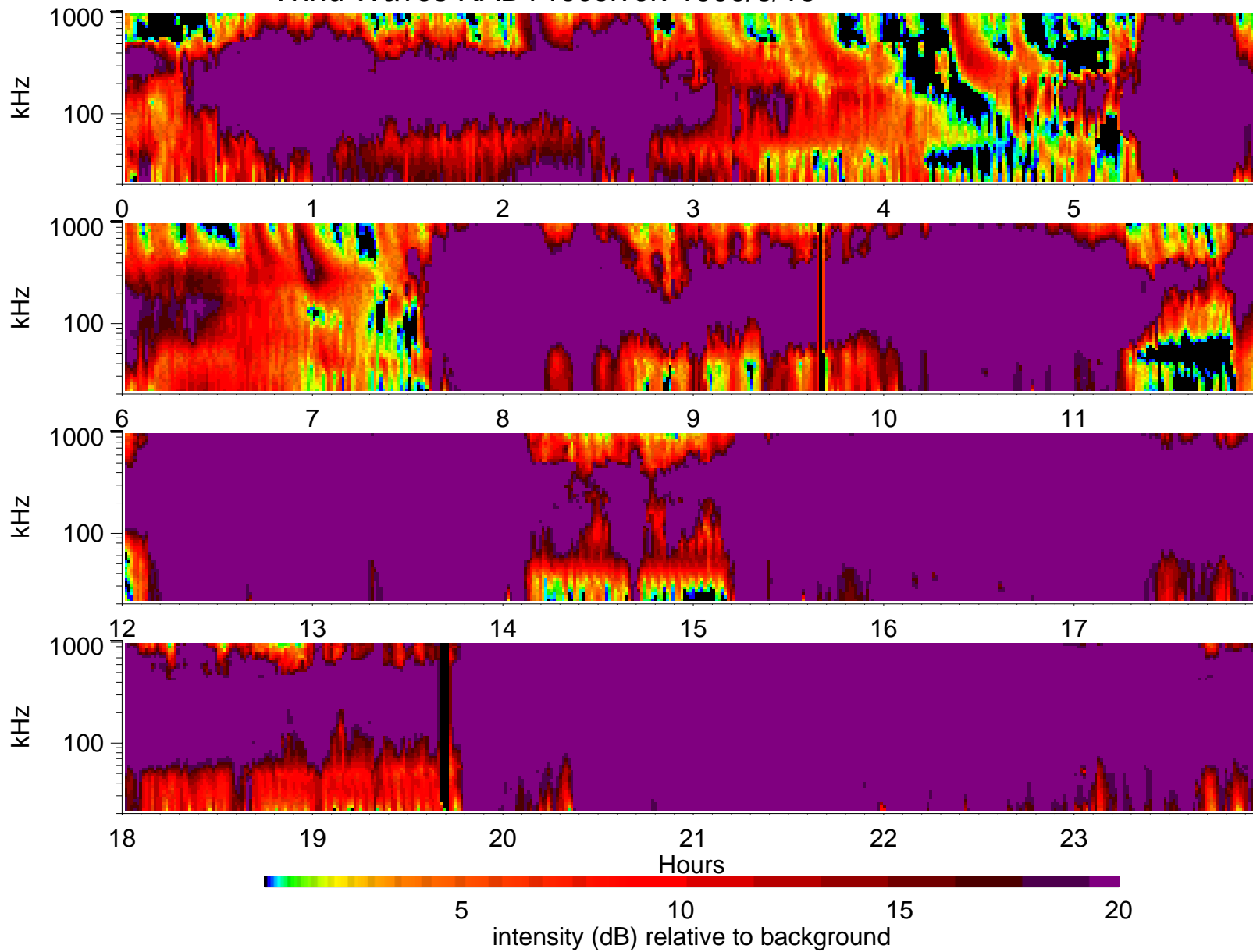
Wind Waves RAD1 receiver: 1999/8/18
