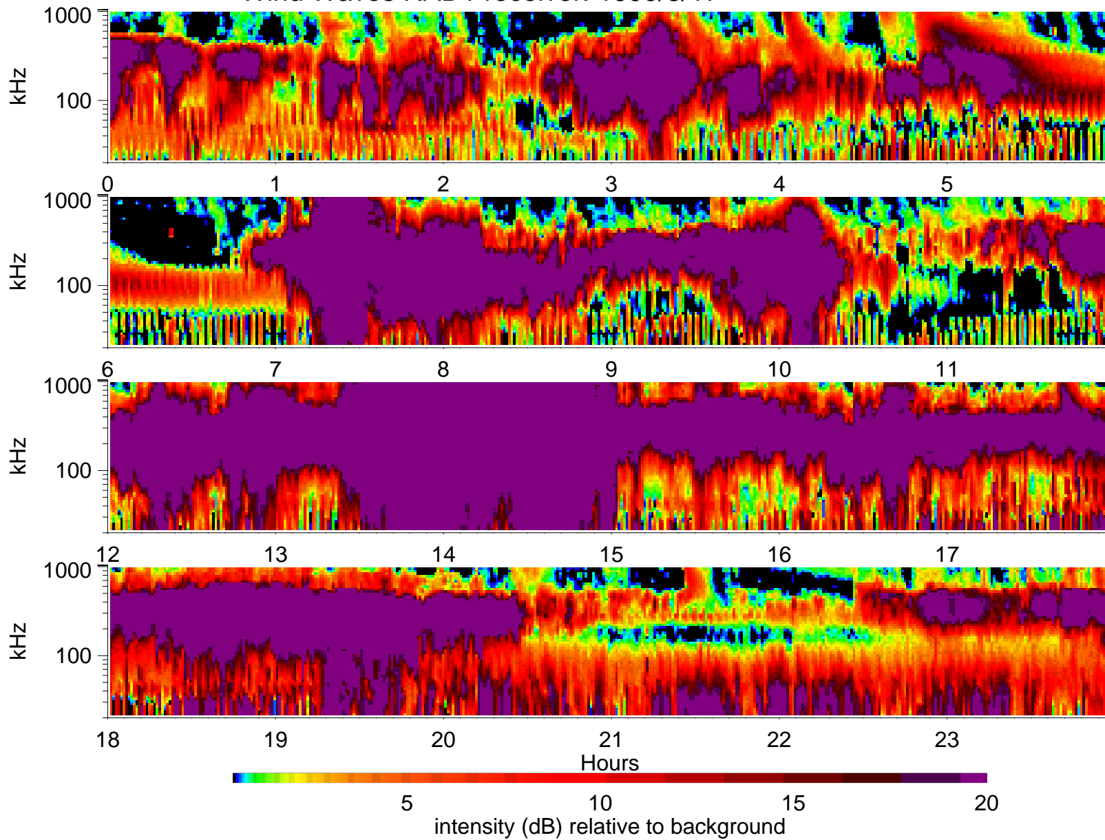
Wind Waves RAD1 receiver: 1999/8/17
