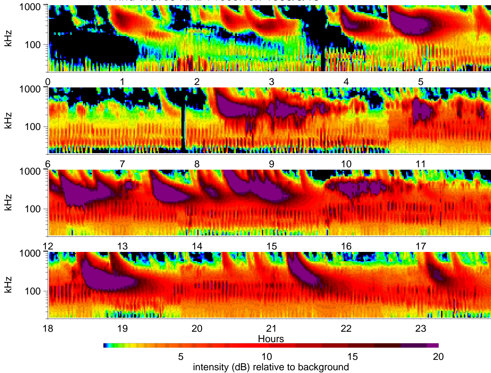
Wind Waves RAD1 receiver: 1999/8/15
