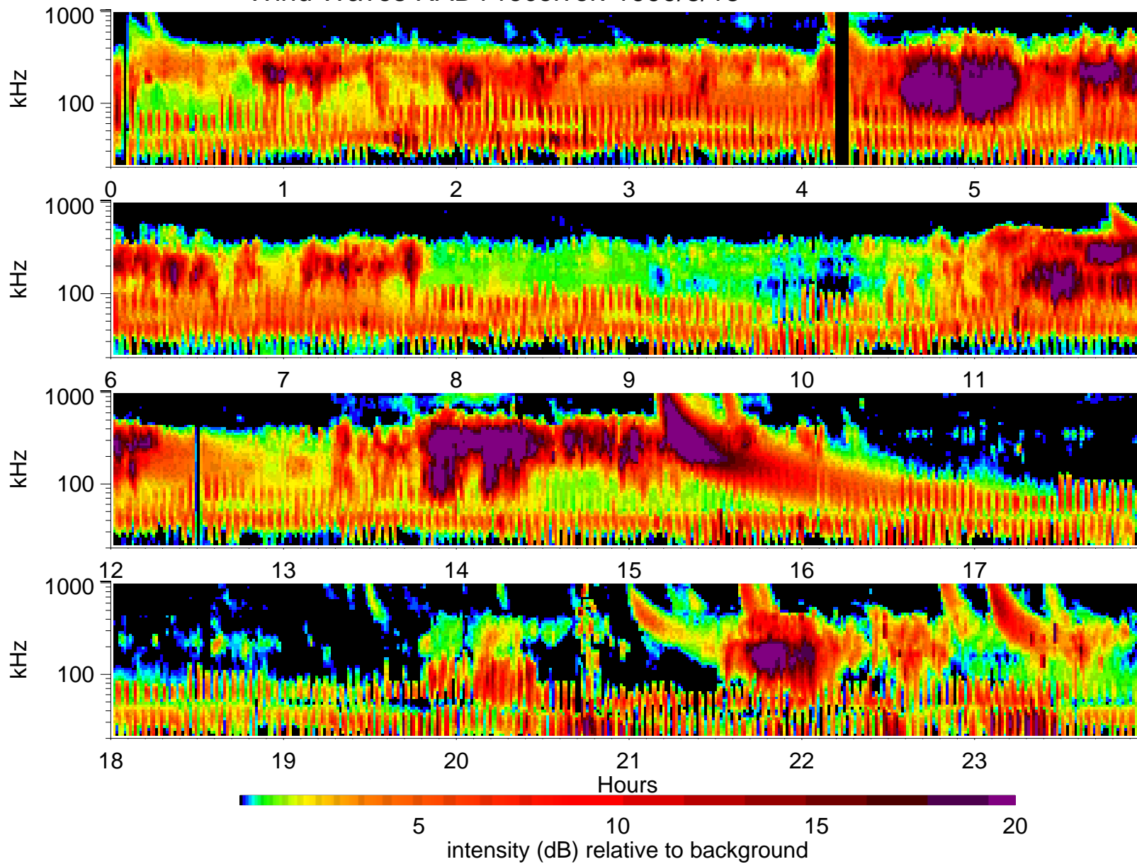
Wind Waves RAD1 receiver: 1999/8/13
