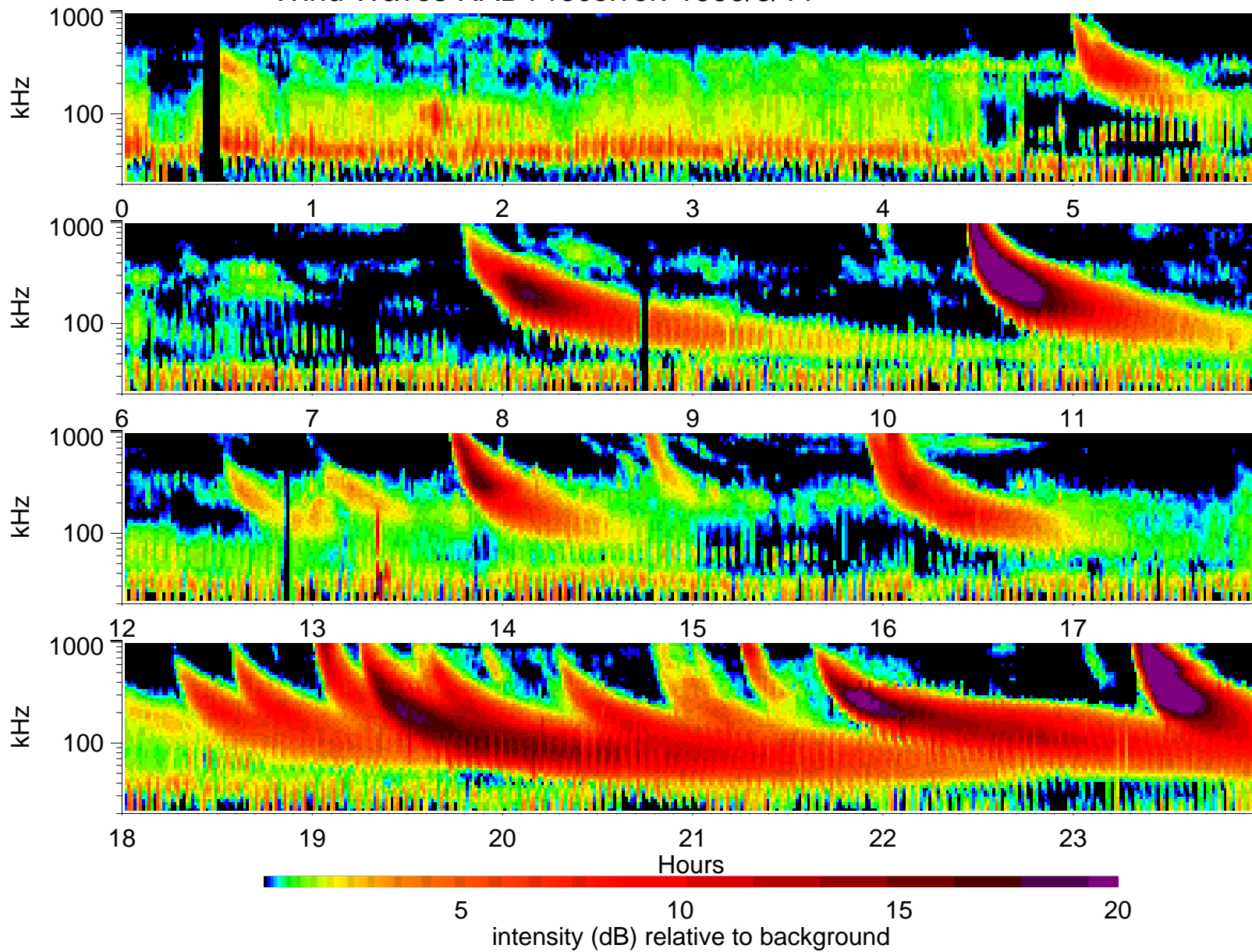
Wind Waves RAD1 receiver: 1999/8/11
