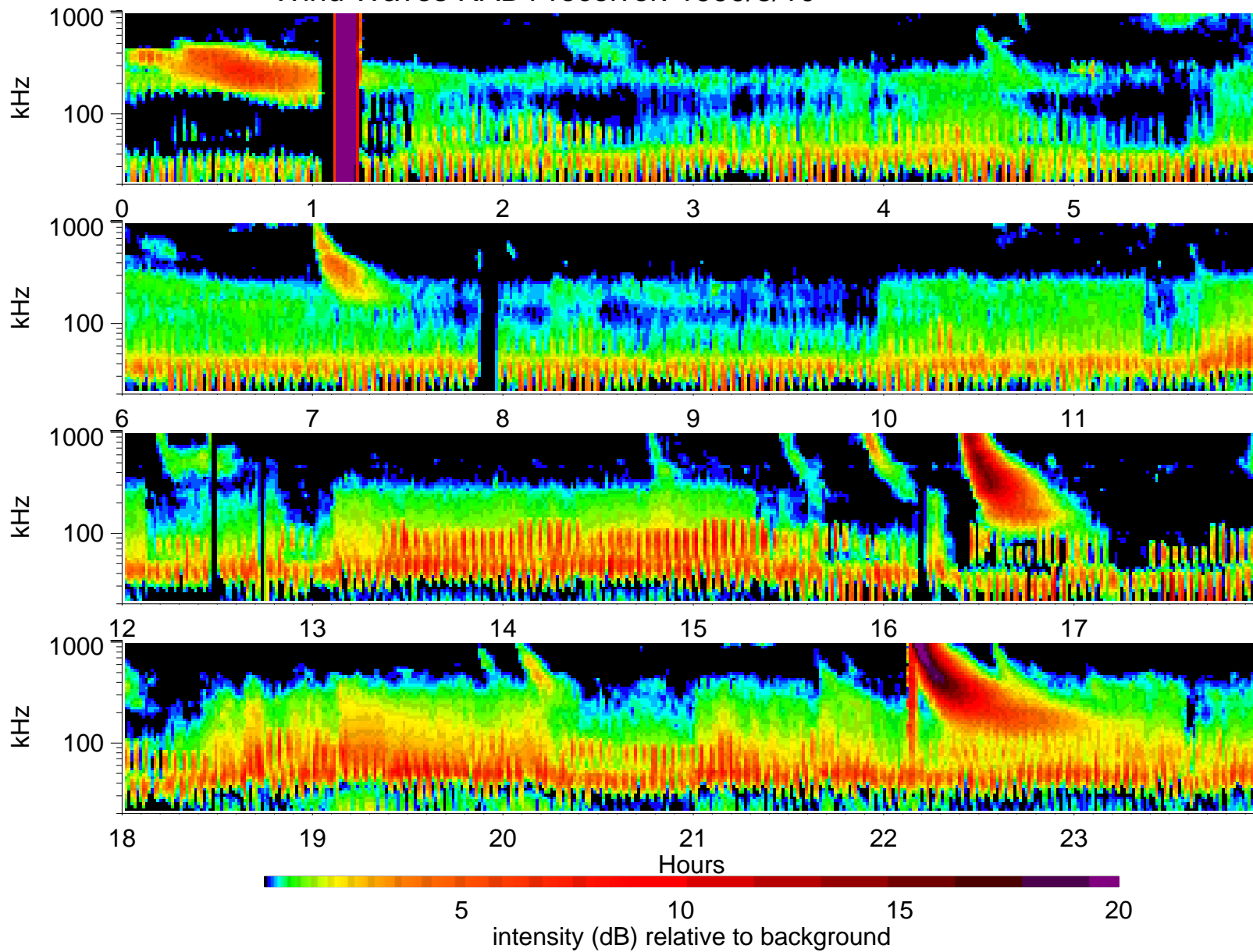
Wind Waves RAD1 receiver: 1999/8/10
