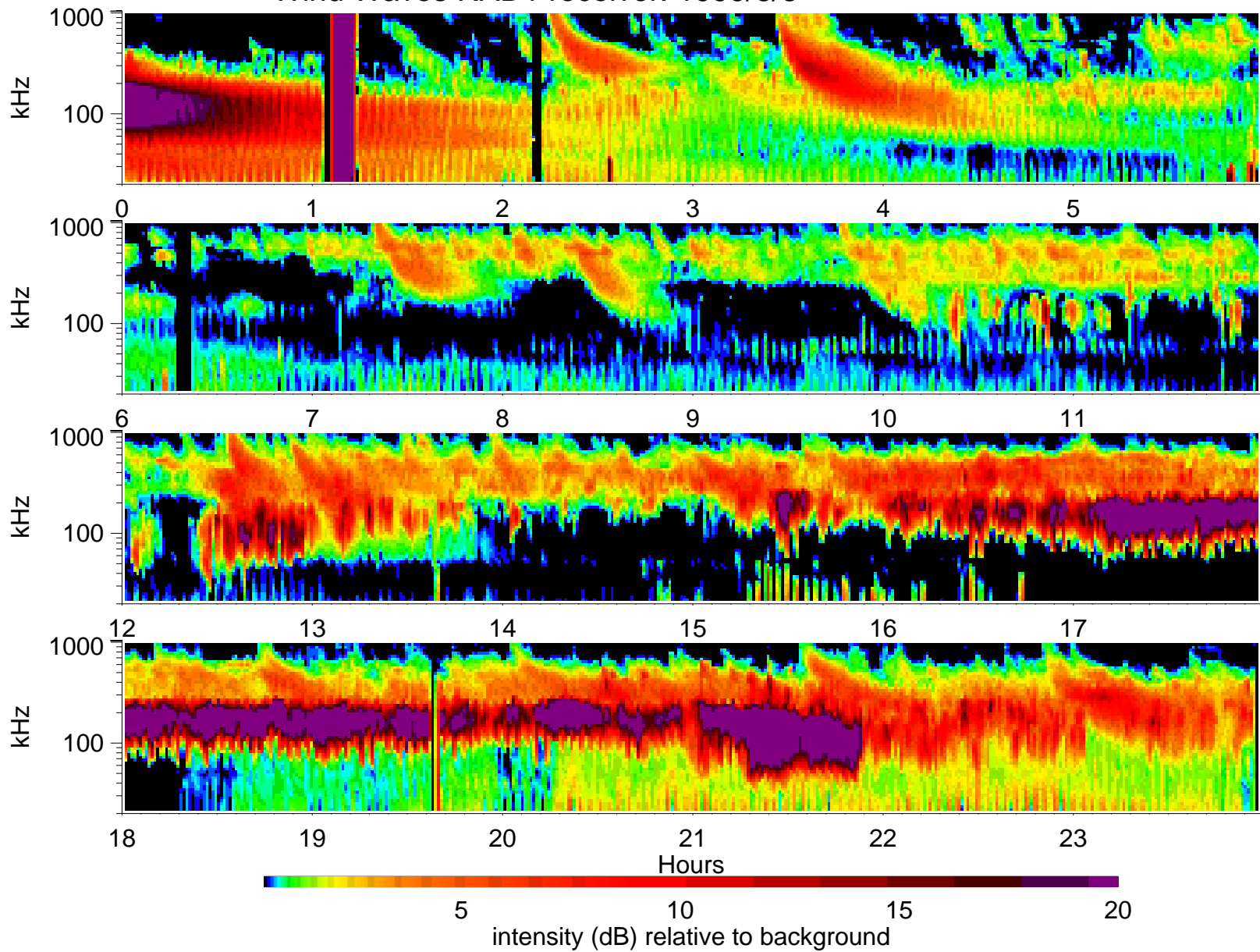
Wind Waves RAD1 receiver: 1999/8/8
