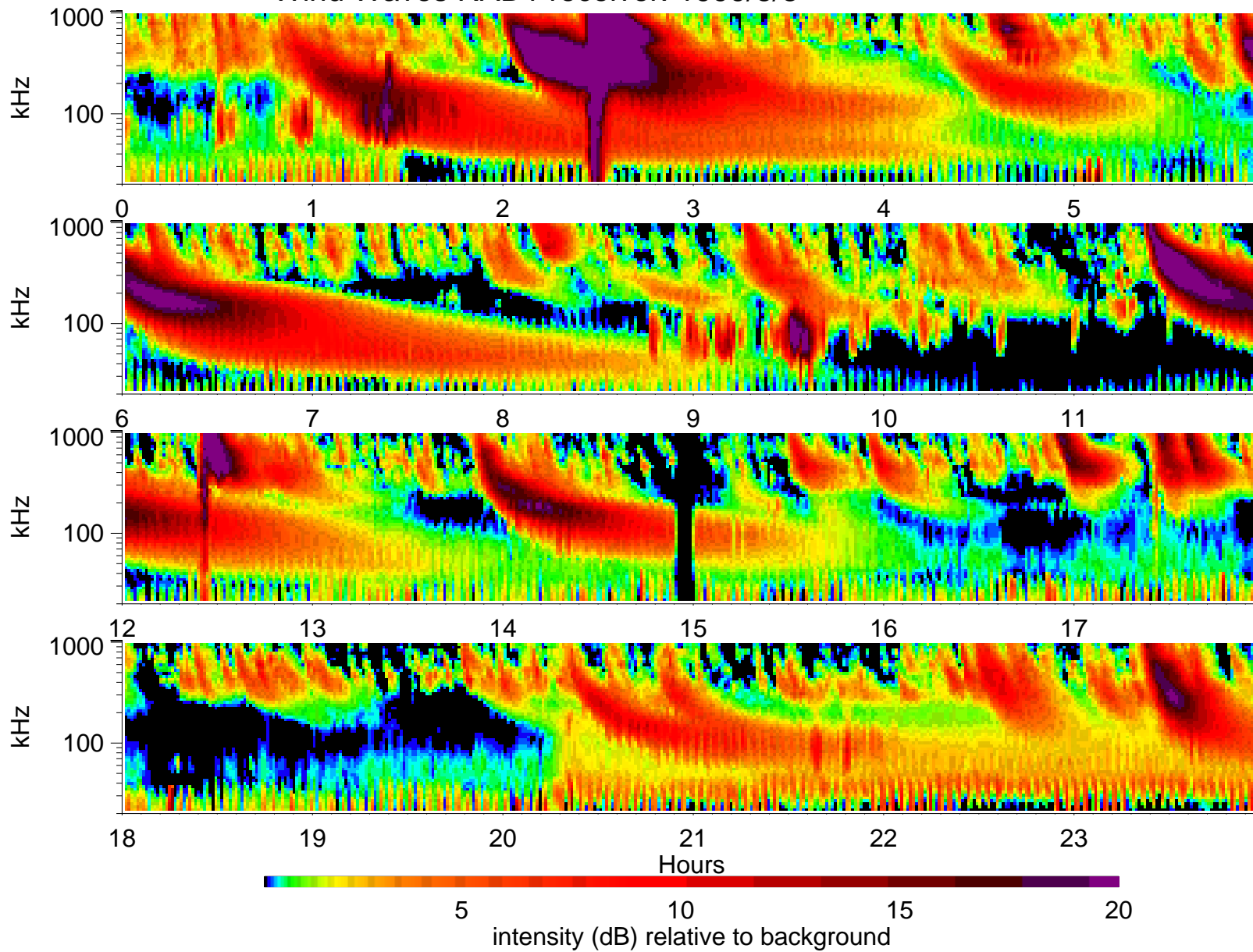
Wind Waves RAD1 receiver: 1999/8/3
