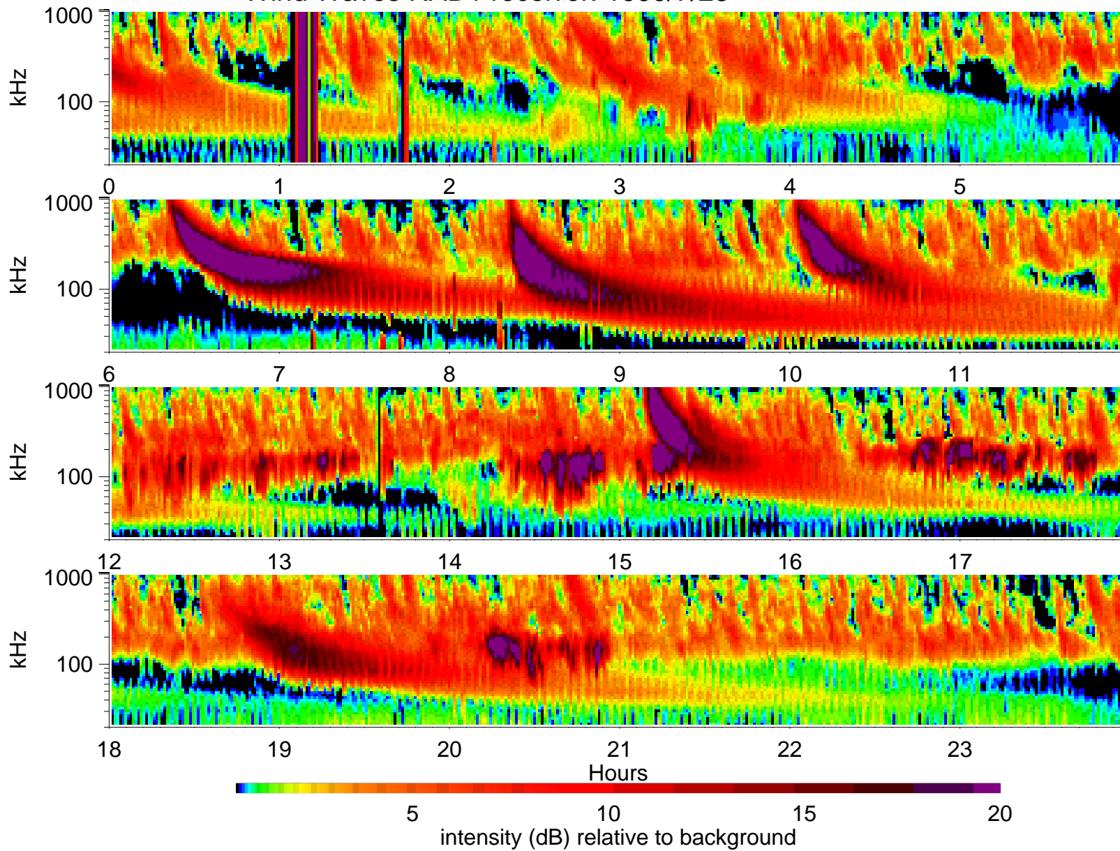
Wind Waves RAD1 receiver: 1999/7/23
