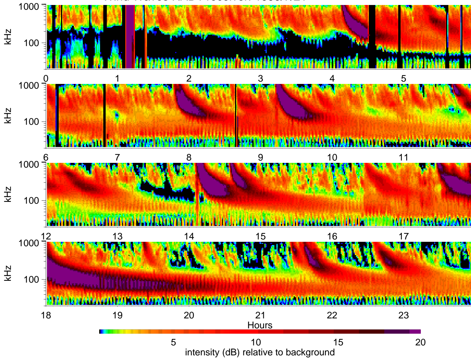
Wind Waves RAD1 receiver: 1999/7/21
