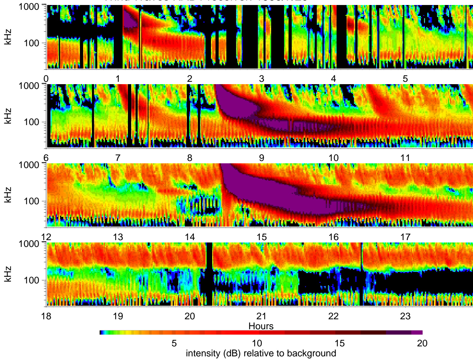
Wind Waves RAD1 receiver: 1999/7/20
