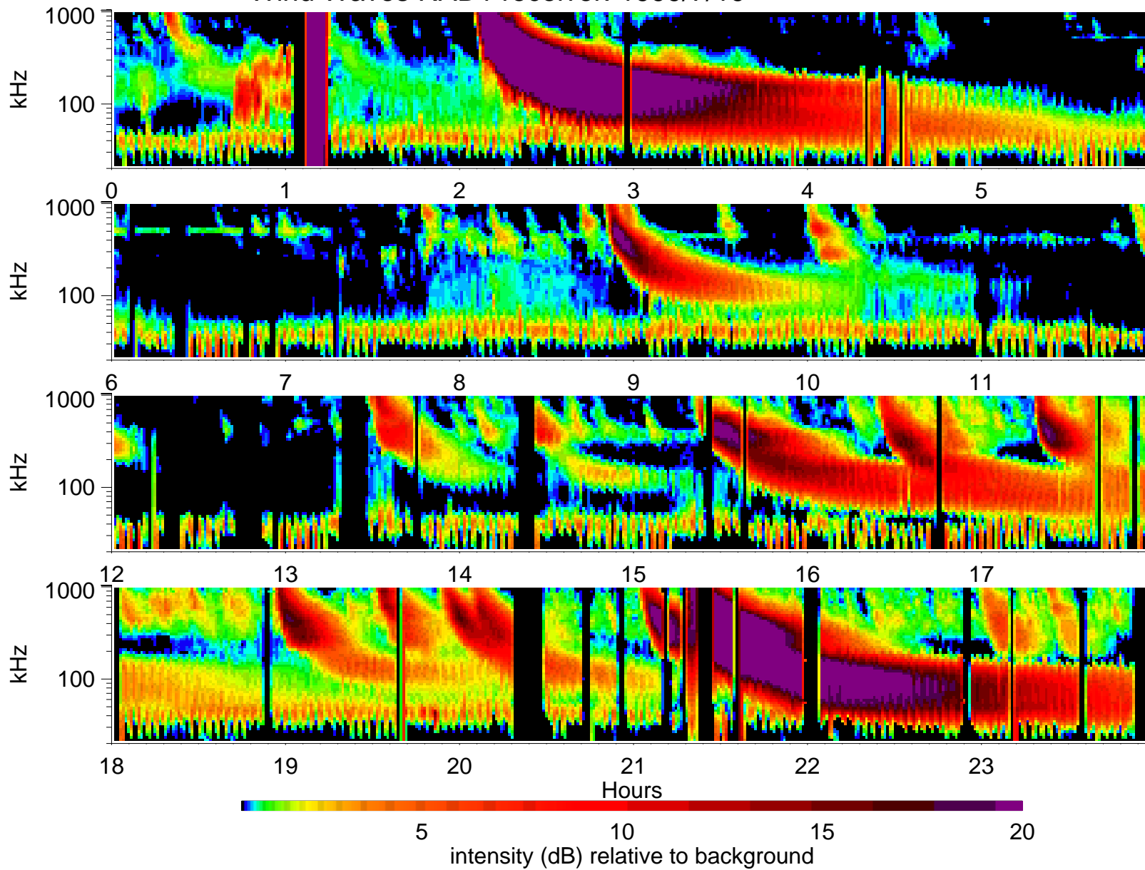
Wind Waves RAD1 receiver: 1999/7/19
