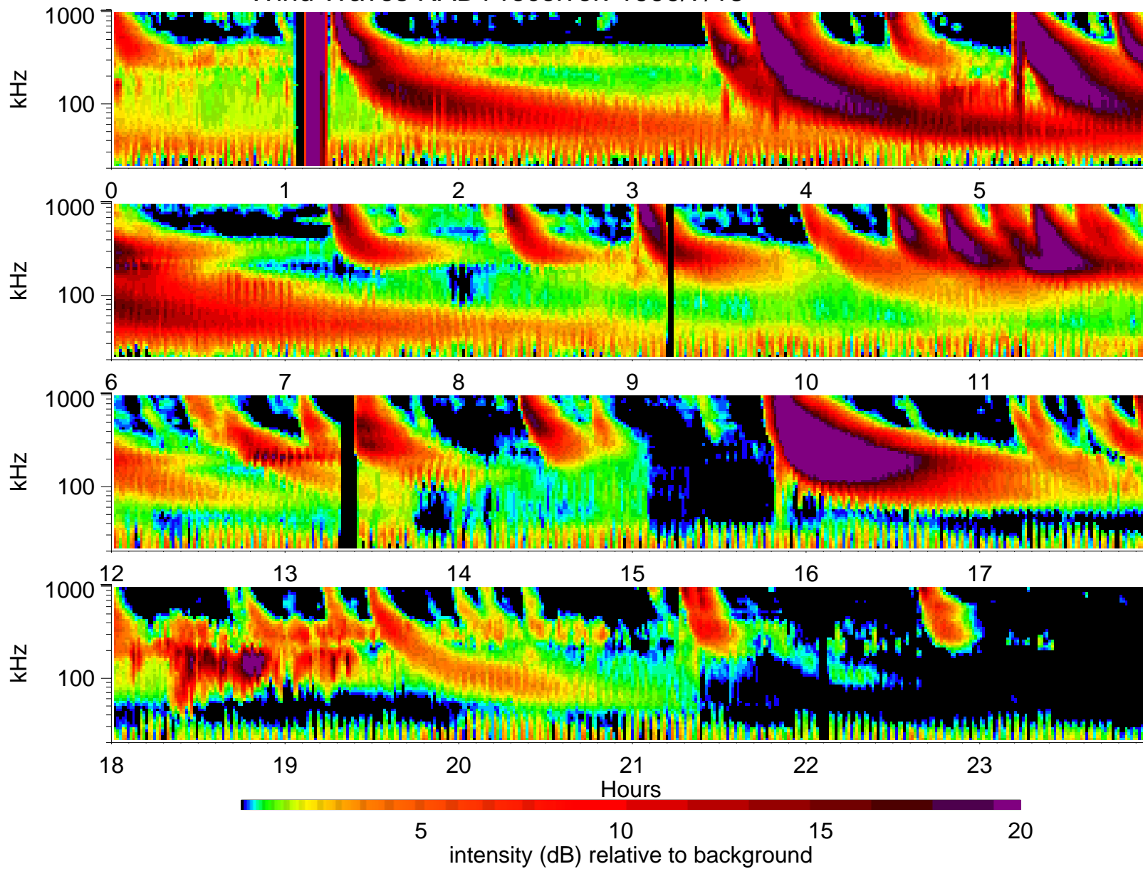
Wind Waves RAD1 receiver: 1999/7/13
