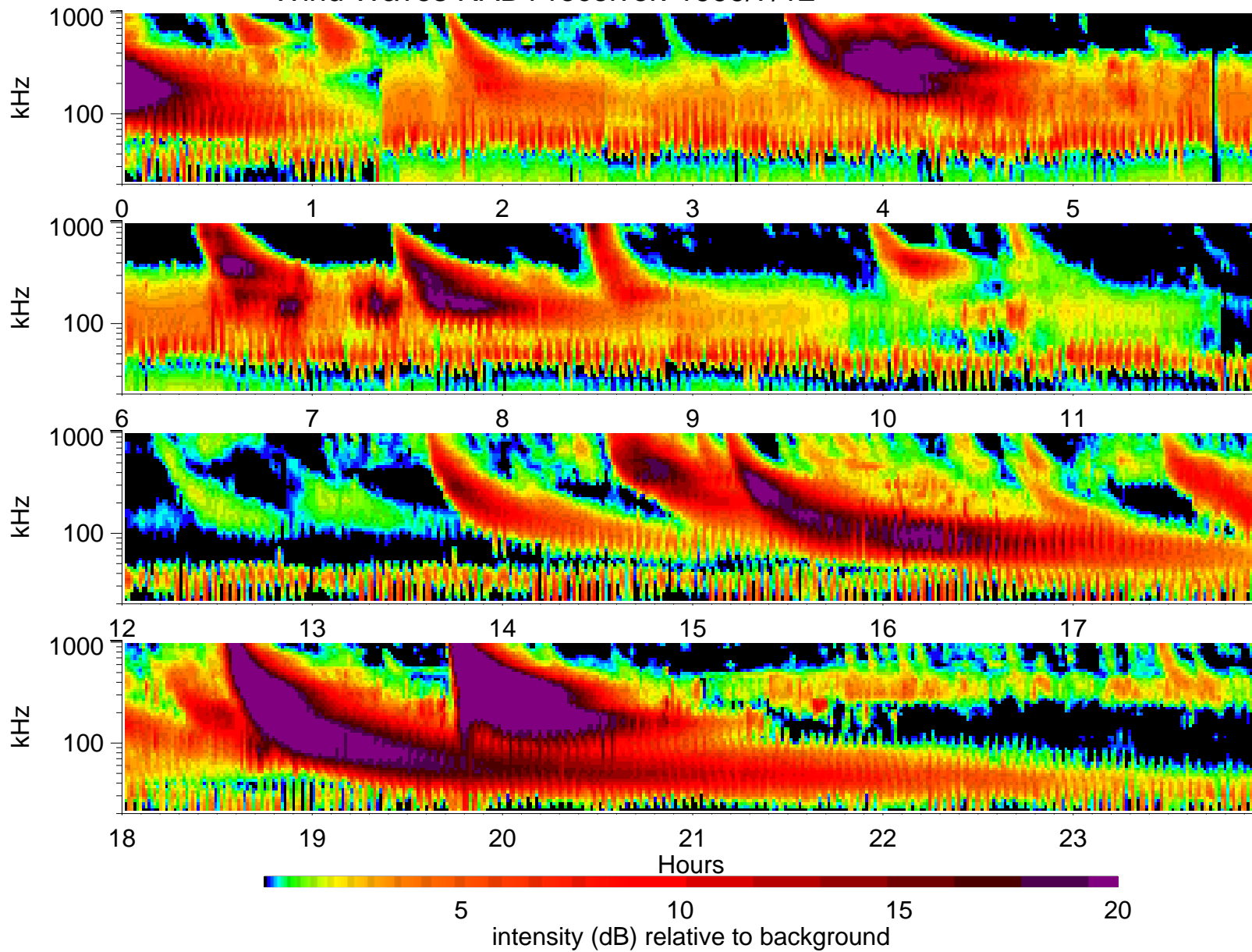
Wind Waves RAD1 receiver: 1999/7/12
