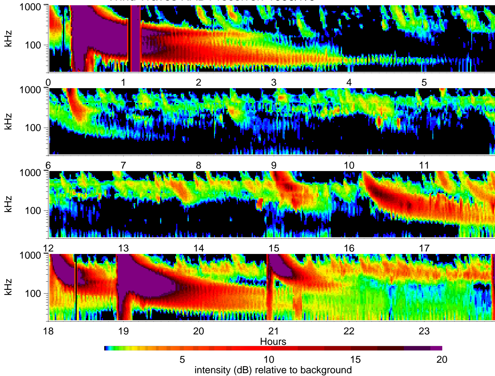
Wind Waves RAD1 receiver: 1999/7/9
