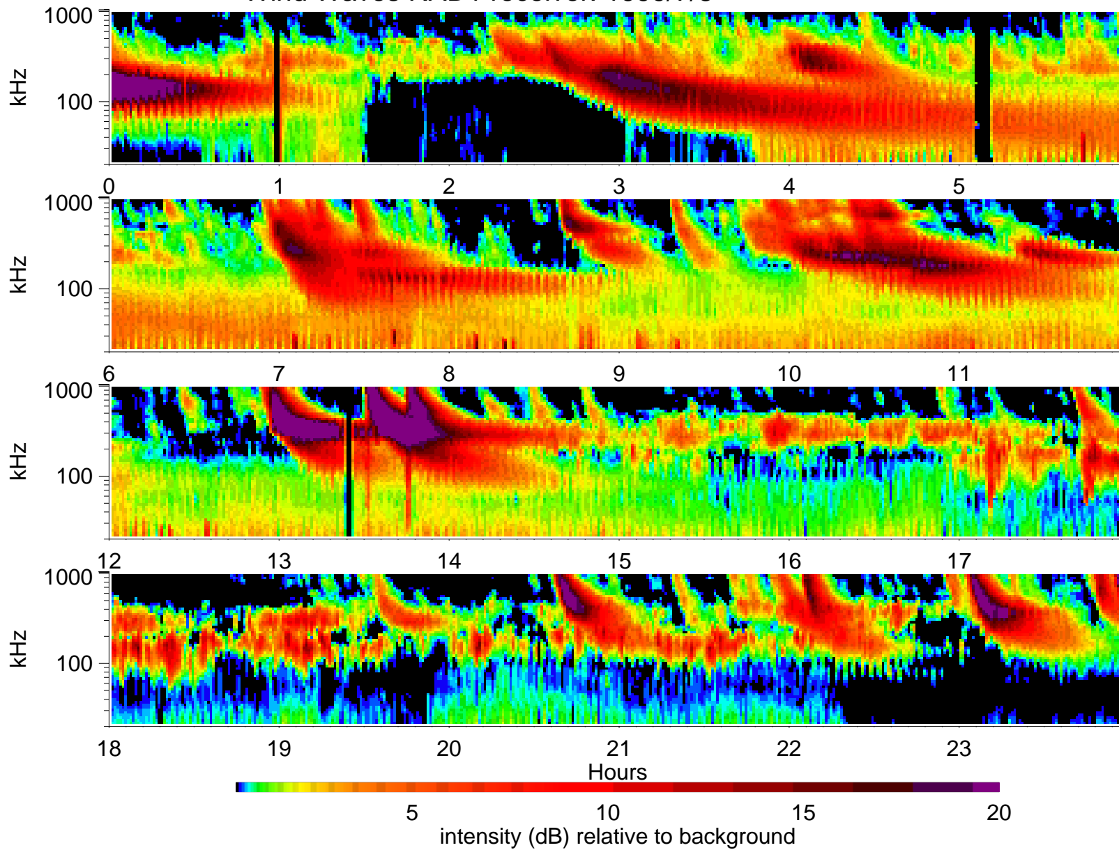
Wind Waves RAD1 receiver: 1999/7/8
