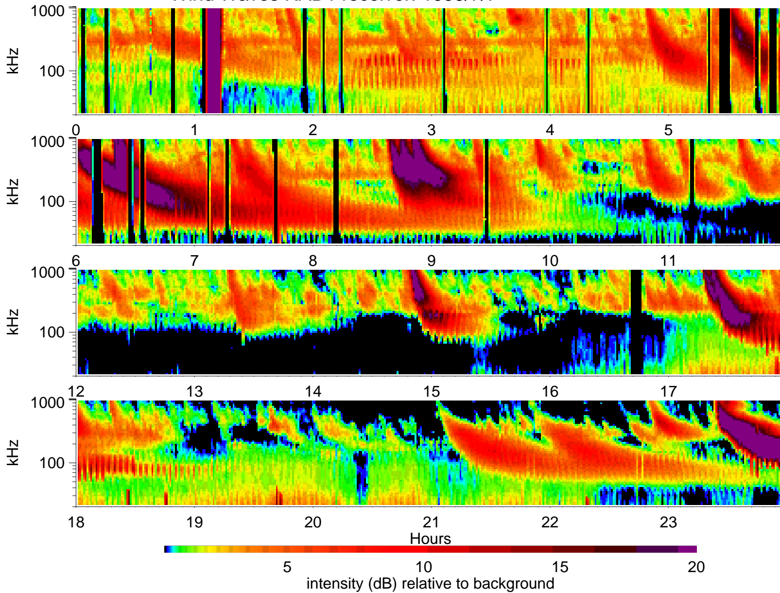
Wind Waves RAD1 receiver: 1999/7/7
