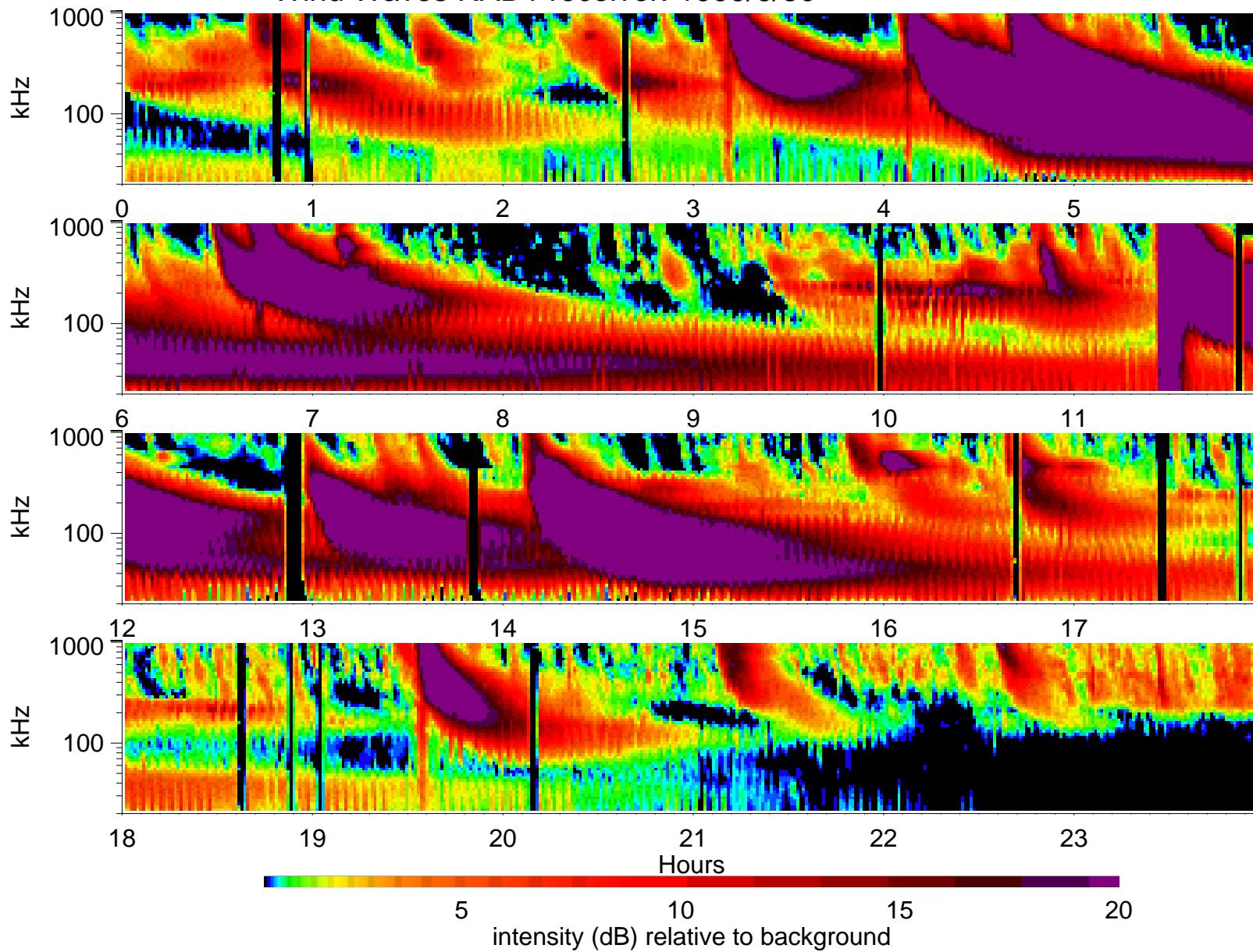
Wind Waves RAD1 receiver: 1999/6/30
