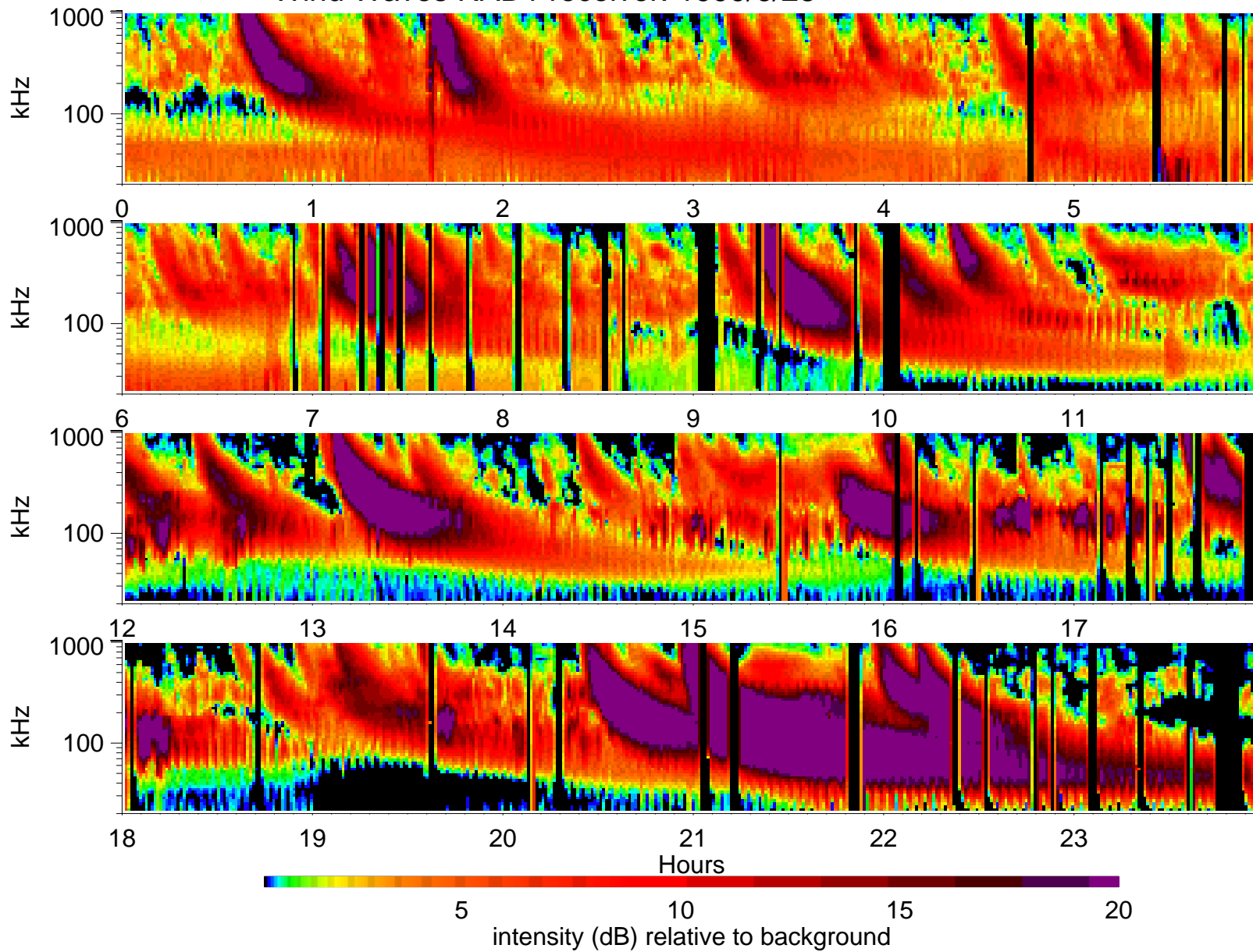
Wind Waves RAD1 receiver: 1999/6/28
