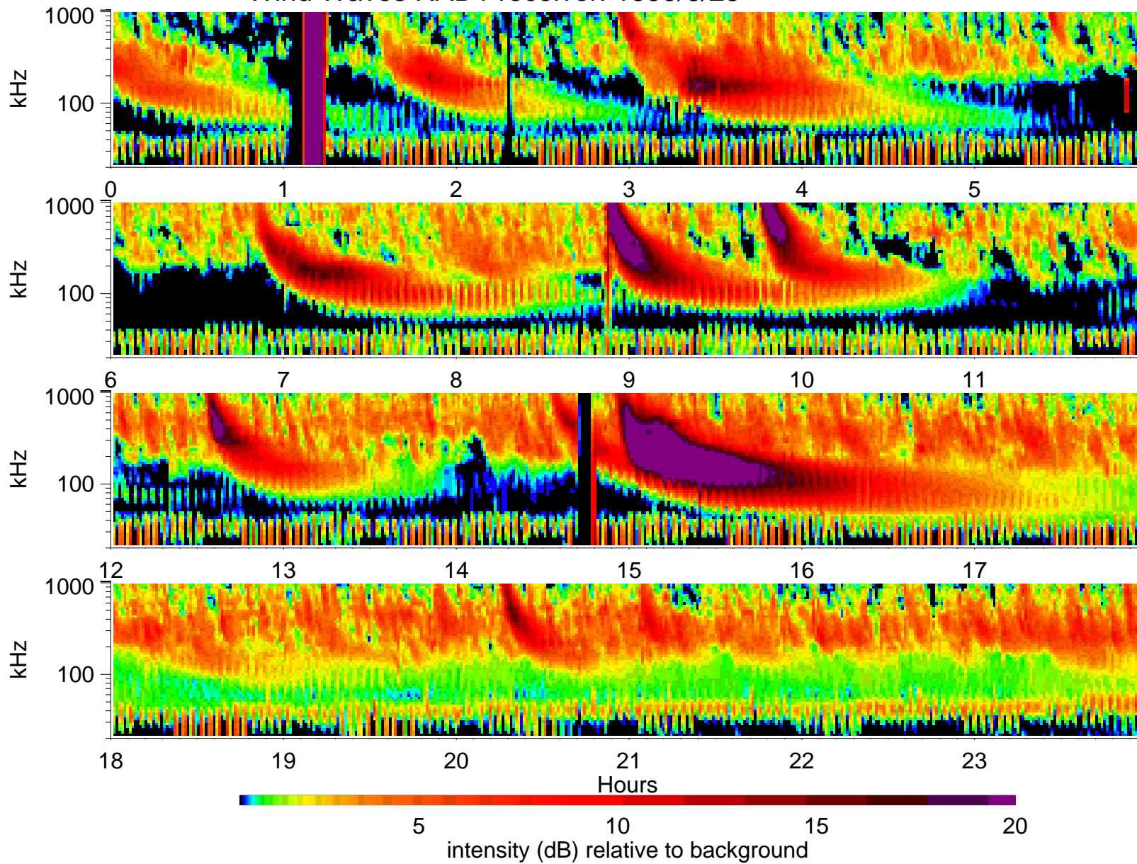
Wind Waves RAD1 receiver: 1999/6/25
