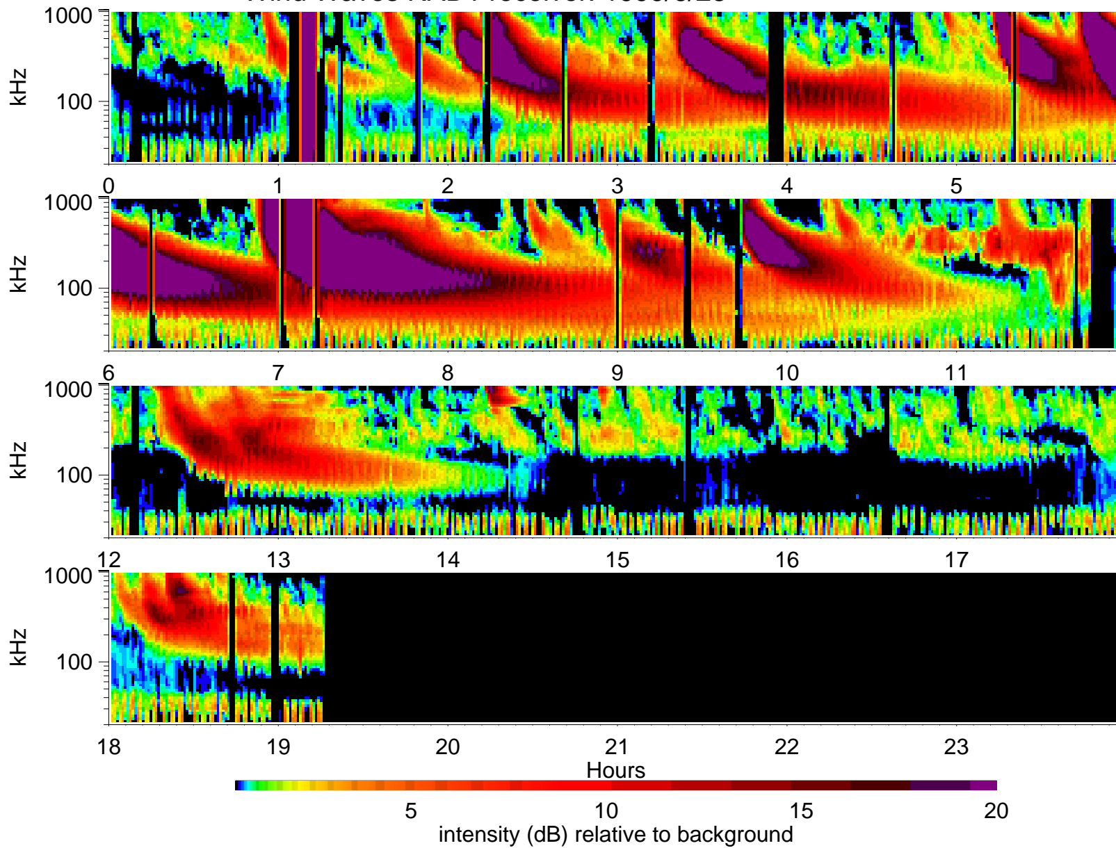
Wind Waves RAD1 receiver: 1999/6/23
