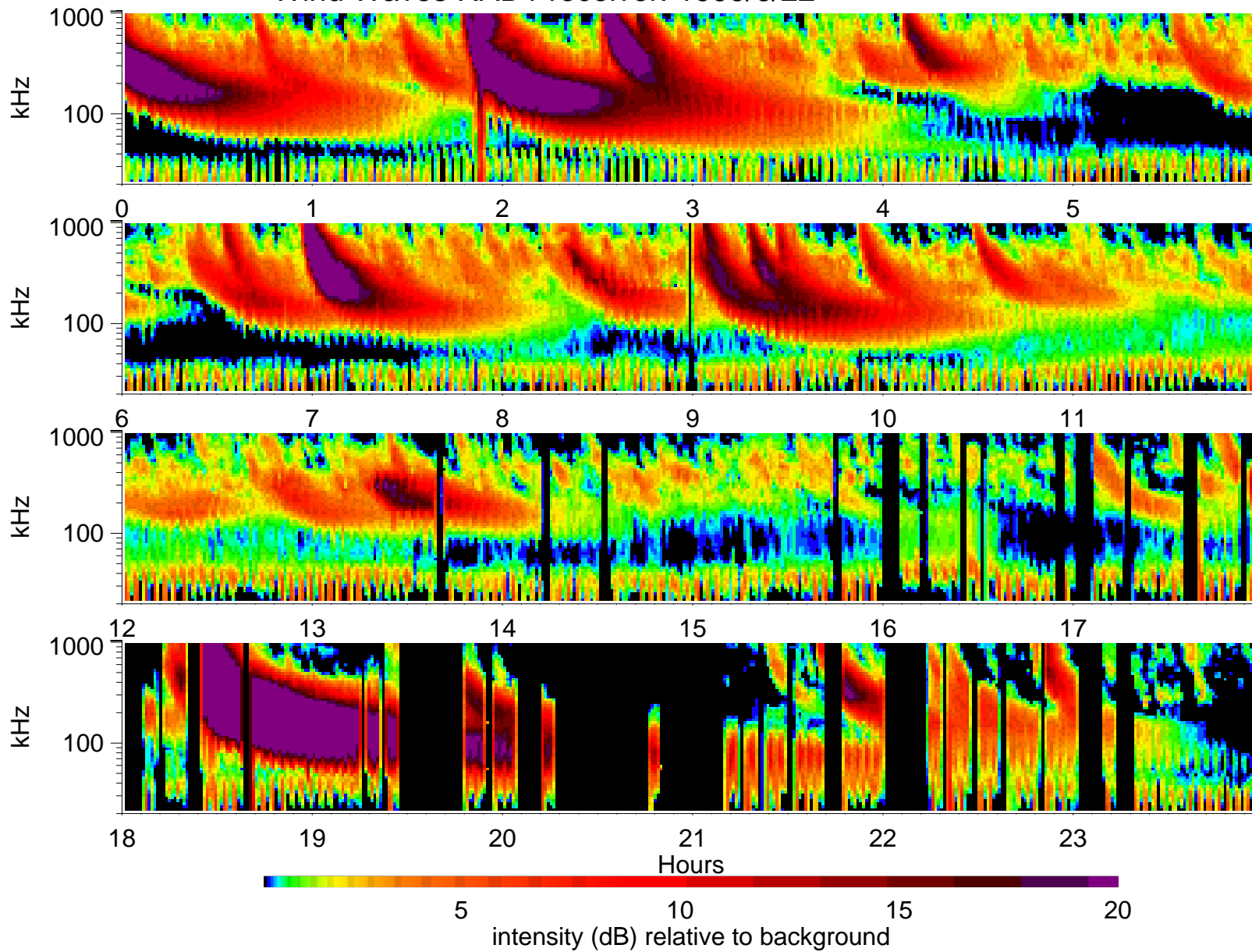
Wind Waves RAD1 receiver: 1999/6/22
