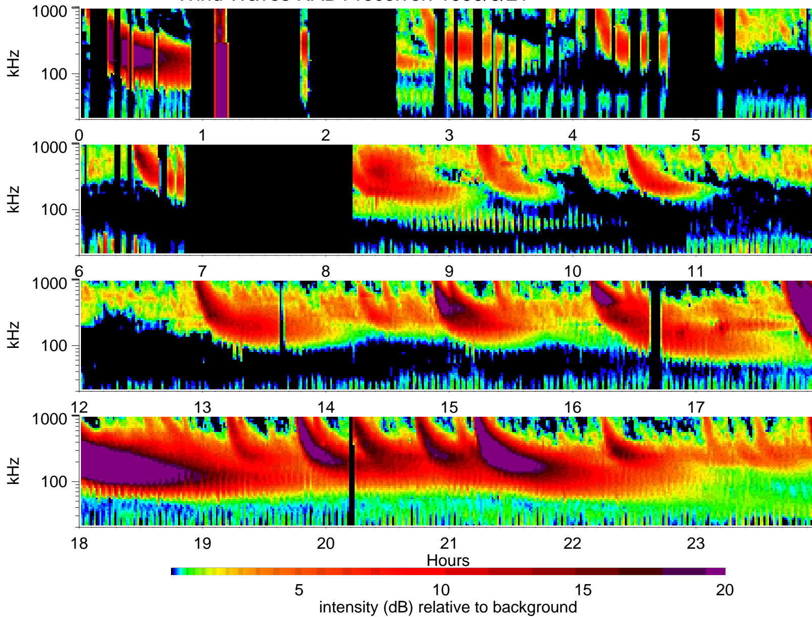
Wind Waves RAD1 receiver: 1999/6/21
