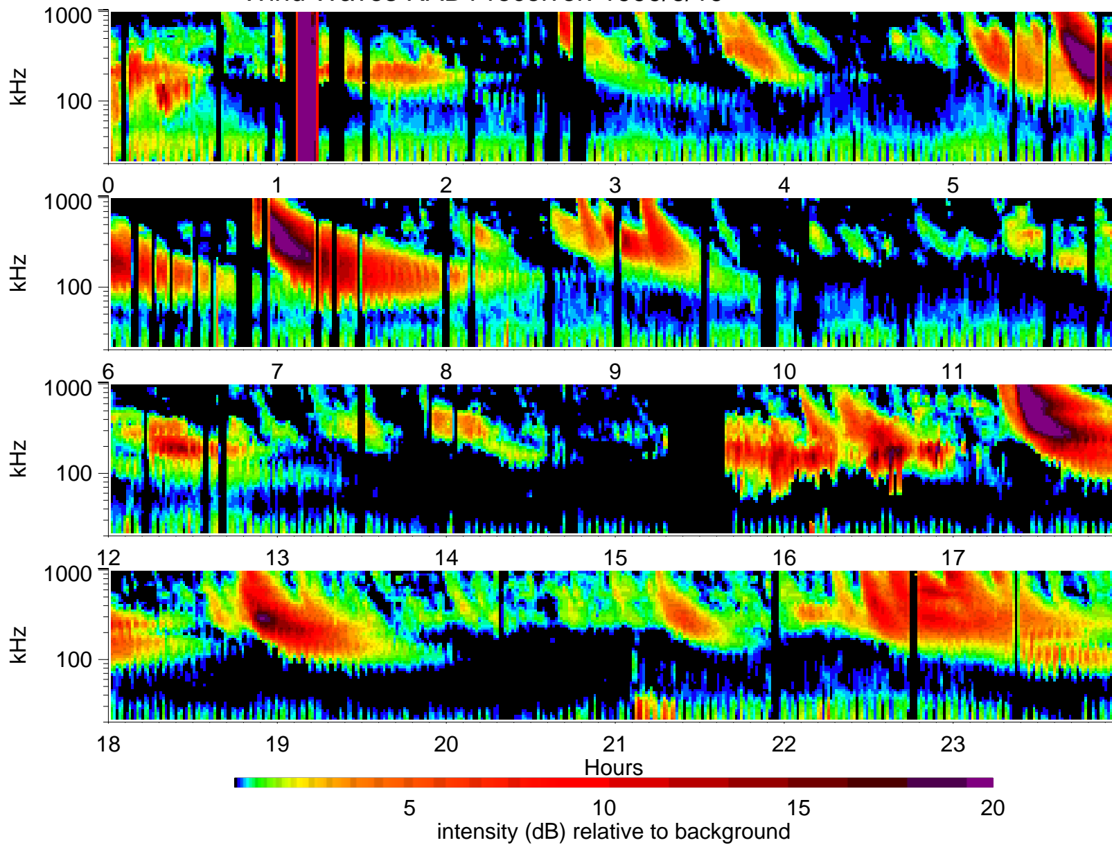
Wind Waves RAD1 receiver: 1999/6/19
